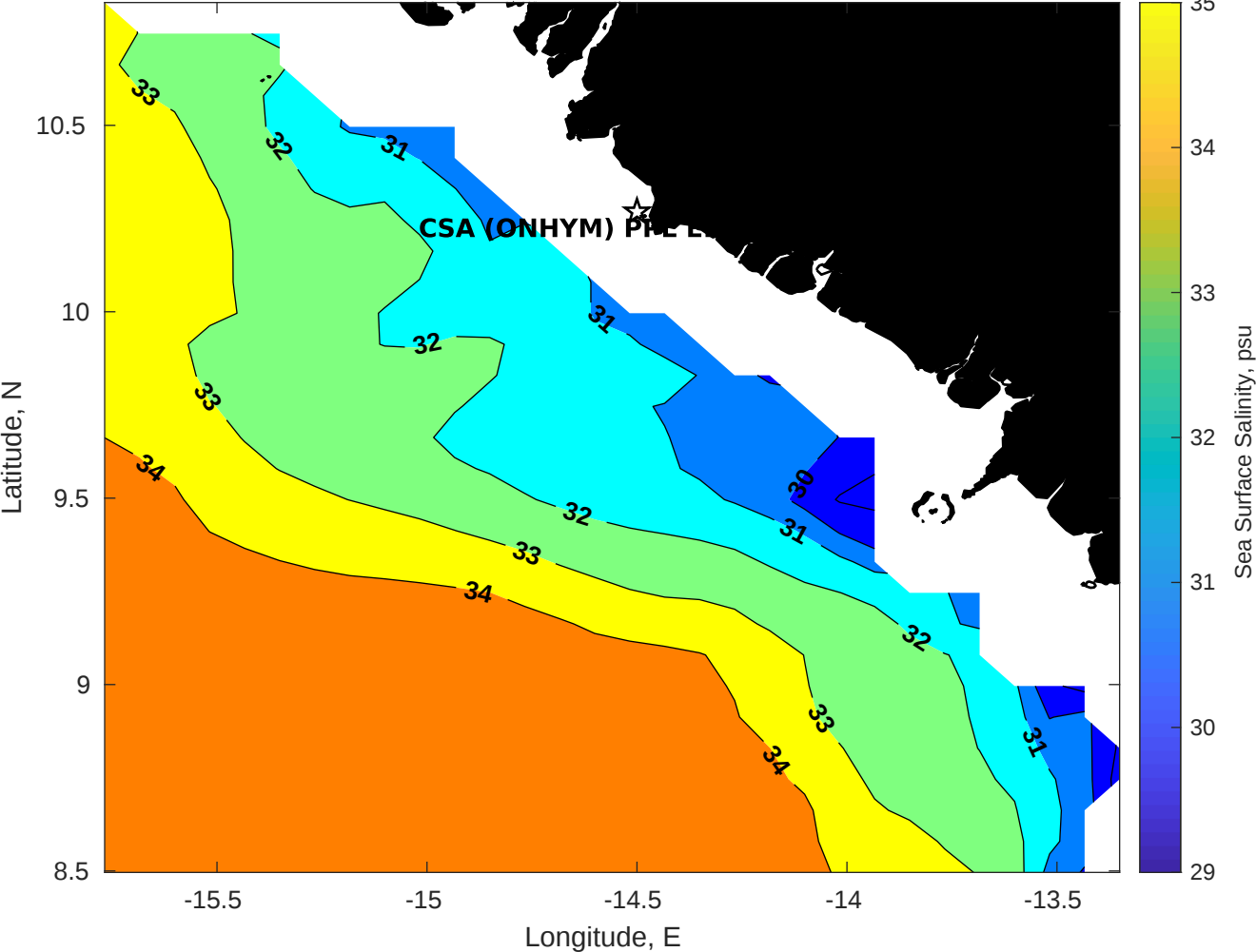
Surface Salinity for CSA (ONHYM) PPL EBS - Guinea at 09-Sep-2025 00:00:00
