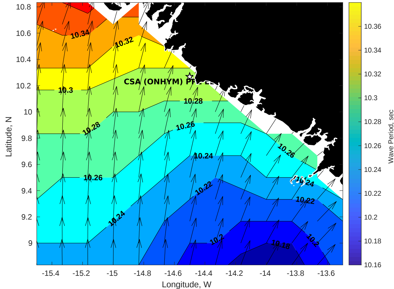
Wave Period (sec) for CSA (ONHYM) PPL EBS - Guinea at 10-Sep-2025 09:00:00
