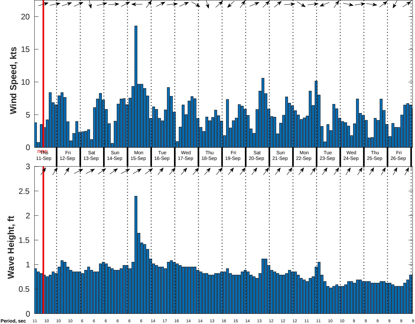
Wind & Wave Forecast for CSA (ONHYM) PPL EBS - Guinea from 10-Sep-2025 01:00:00 to 26-Sep-2025 01:00:00
