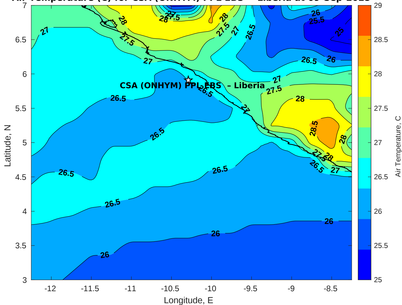
Air Temperature (C) for CSA (ONHYM) PPL EBS - Liberia at 09-Sep-2025
