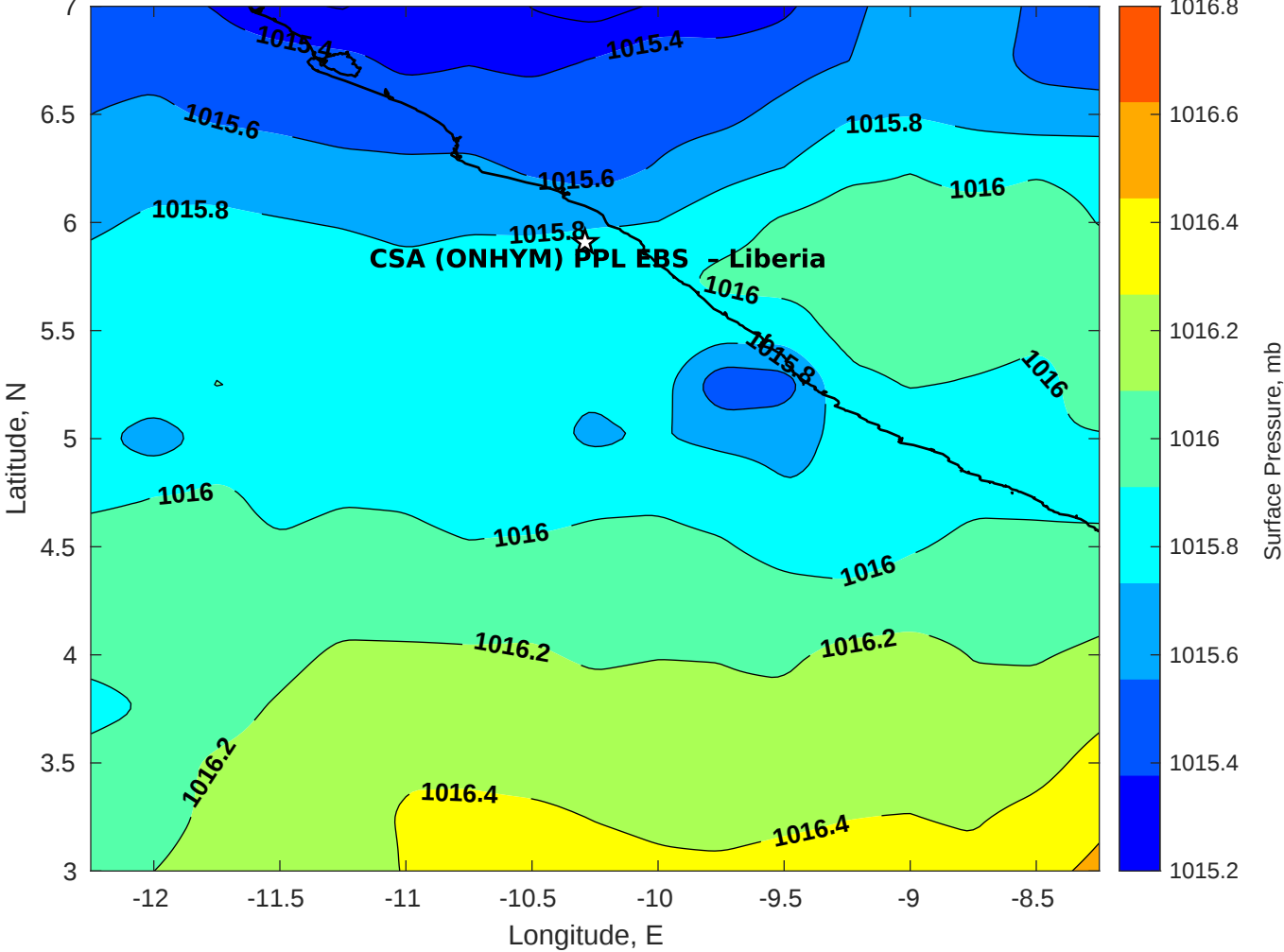
Surface Pressure (mb) for CSA (ONHYM) PPL EBS - Liberia at 10-Sep-2025 12:00:00
