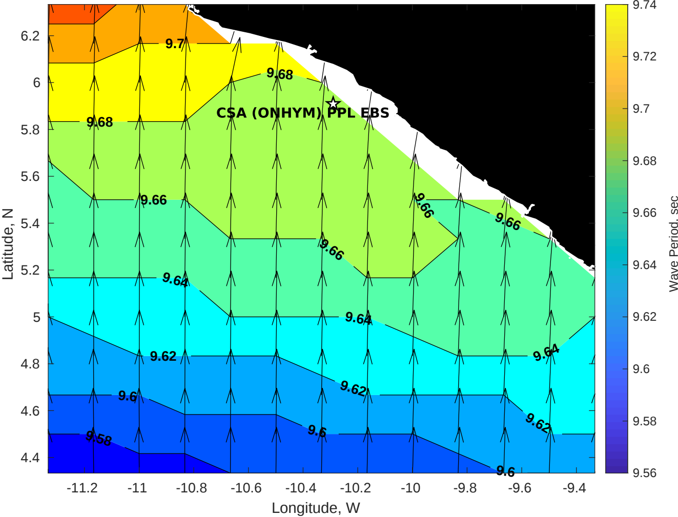
Wave Period (sec) for CSA (ONHYM) PPL EBS - Liberia at 10-Sep-2025 09:00:00
