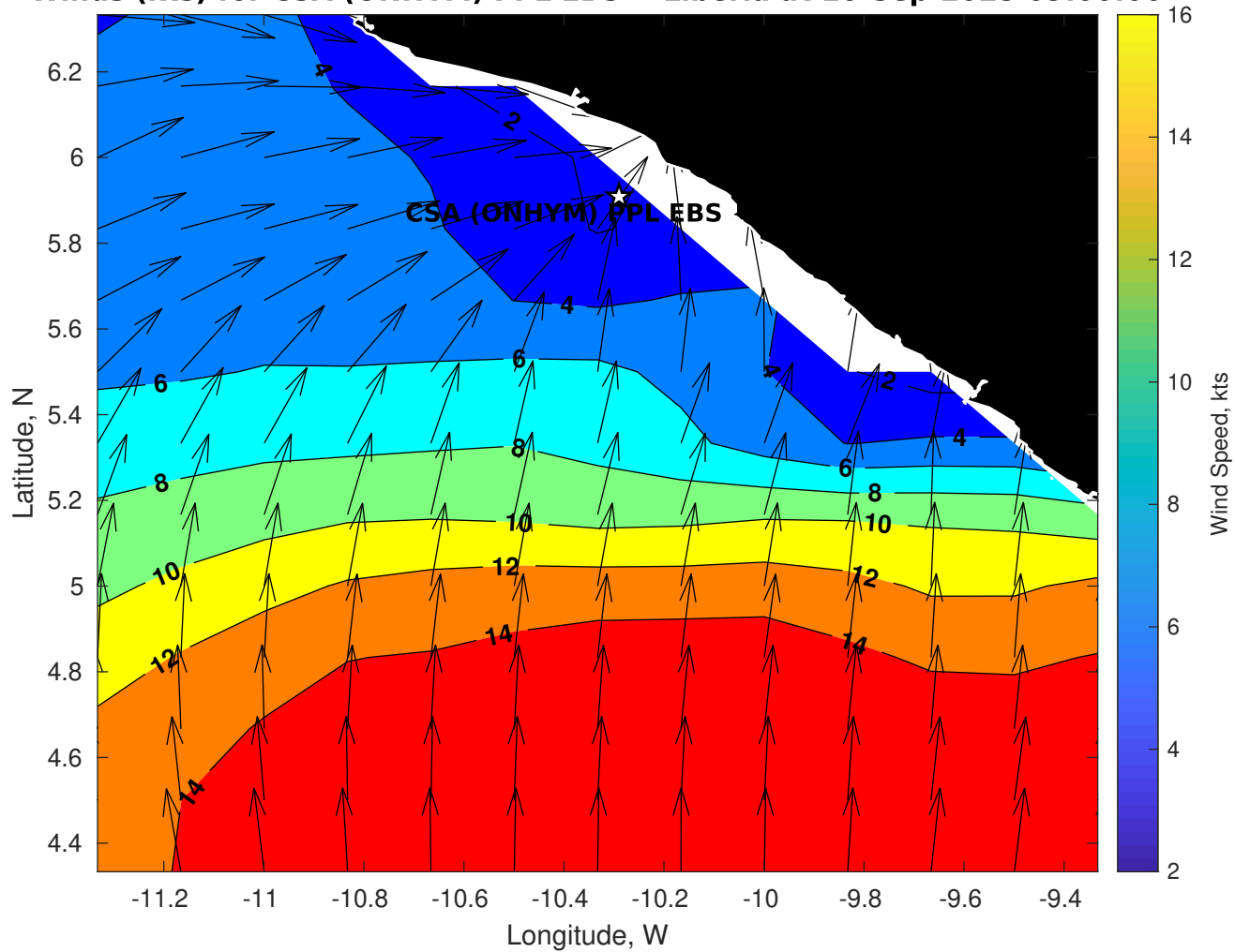
Winds (kts) for CSA (ONHYM) PPL EBS - Liberia at 10-Sep-2025 09:00:00
