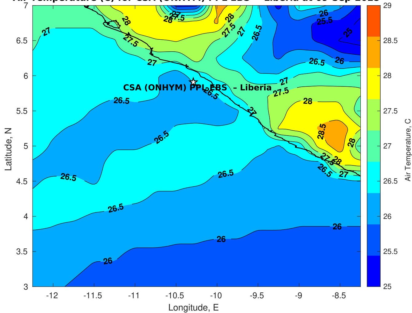
Air Temperature (C) for CSA (ONHYM) PPL EBS - Liberia at 09-Sep-2025
