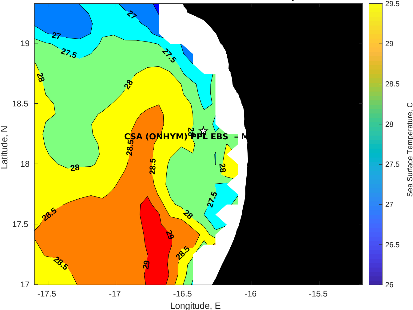
SST for CSA (ONHYM) PPL EBS - Mauritania at 09-Sep-2025 00:00:00
