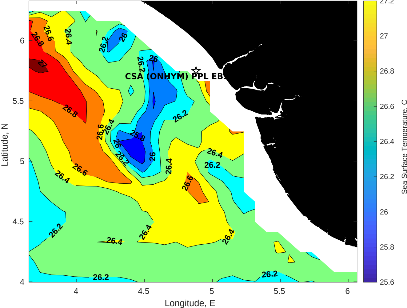
SST for CSA (ONHYM) PPL EBS - Nigeria at 09-Sep-2025 00:00:00
