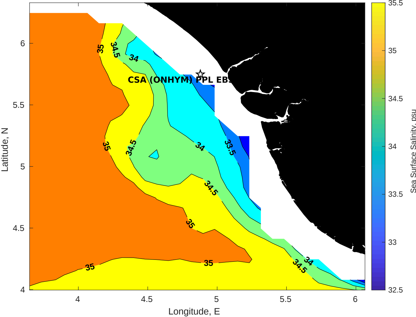
Surface Salinity for CSA (ONHYM) PPL EBS - Nigeria at 09-Sep-2025 00:00:00
