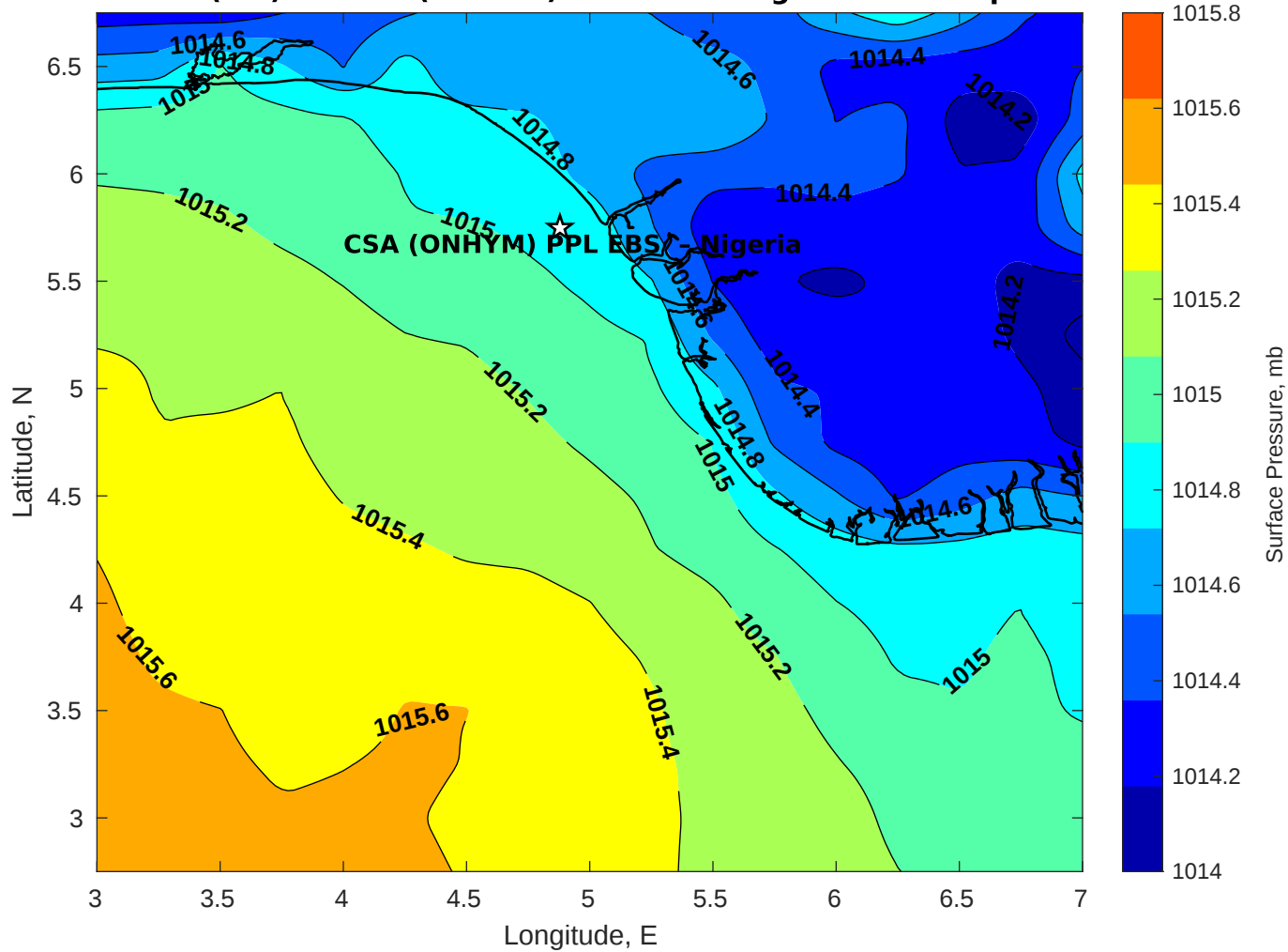
Surface Pressure (mb) for CSA (ONHYM) PPL EBS - Nigeria at 10-Sep-2025 12:00:00
