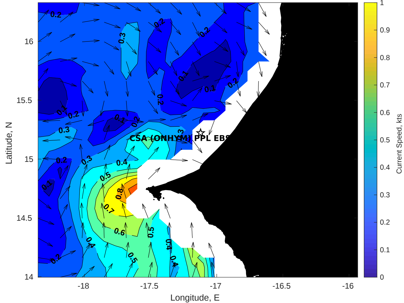
Surface Currents for CSA (ONHYM) PPL EBS - Senegal at 09-Sep-2025 00:00:00
