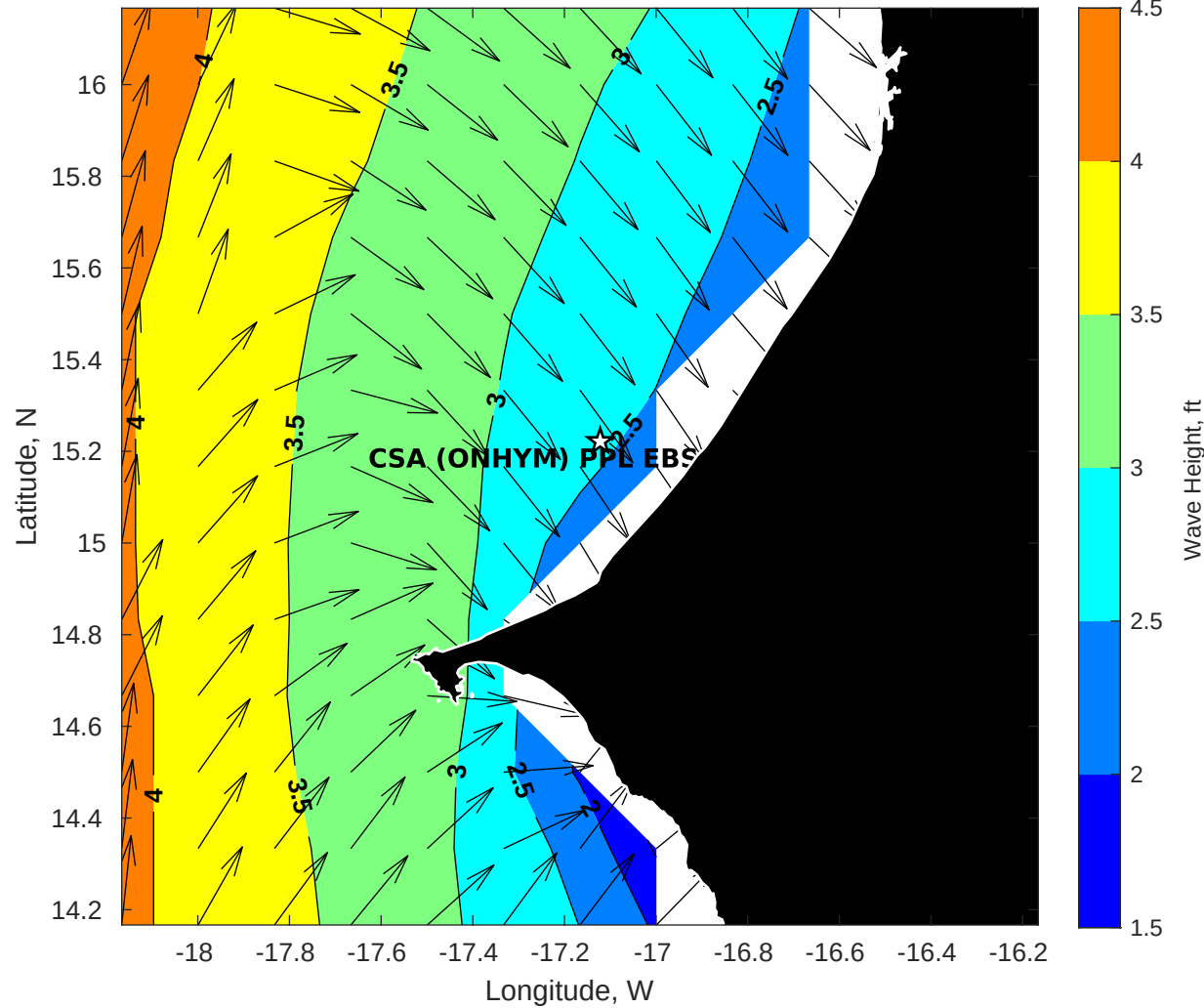
Wave Height (ft) for CSA (ONHYM) PPL EBS - Senegal at 10-Sep-2025 09:00:00
