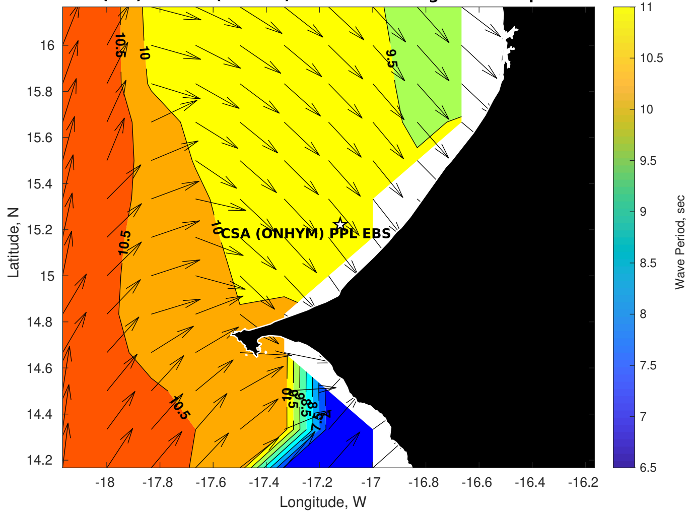
Wave Period (sec) for CSA (ONHYM) PPL EBS - Senegal at 10-Sep-2025 09:00:00
