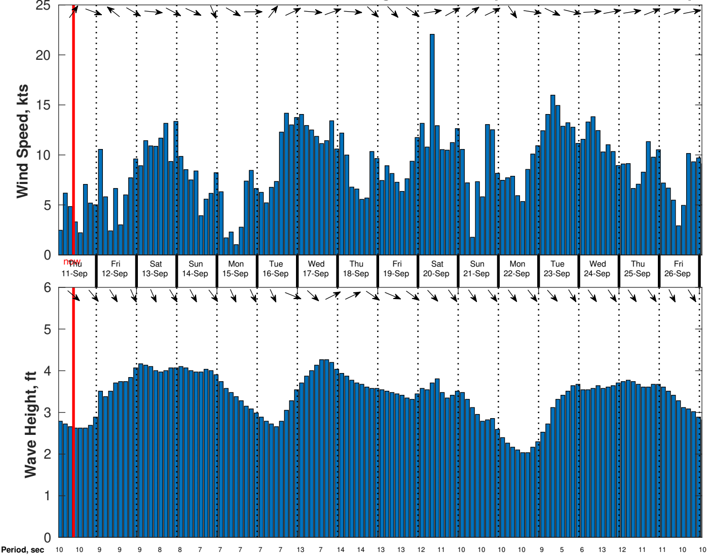
Wind & Wave Forecast for CSA (ONHYM) PPL EBS - Senegal from 10-Sep-2025 01:00:00 to 26-Sep-2025 01:00:00
