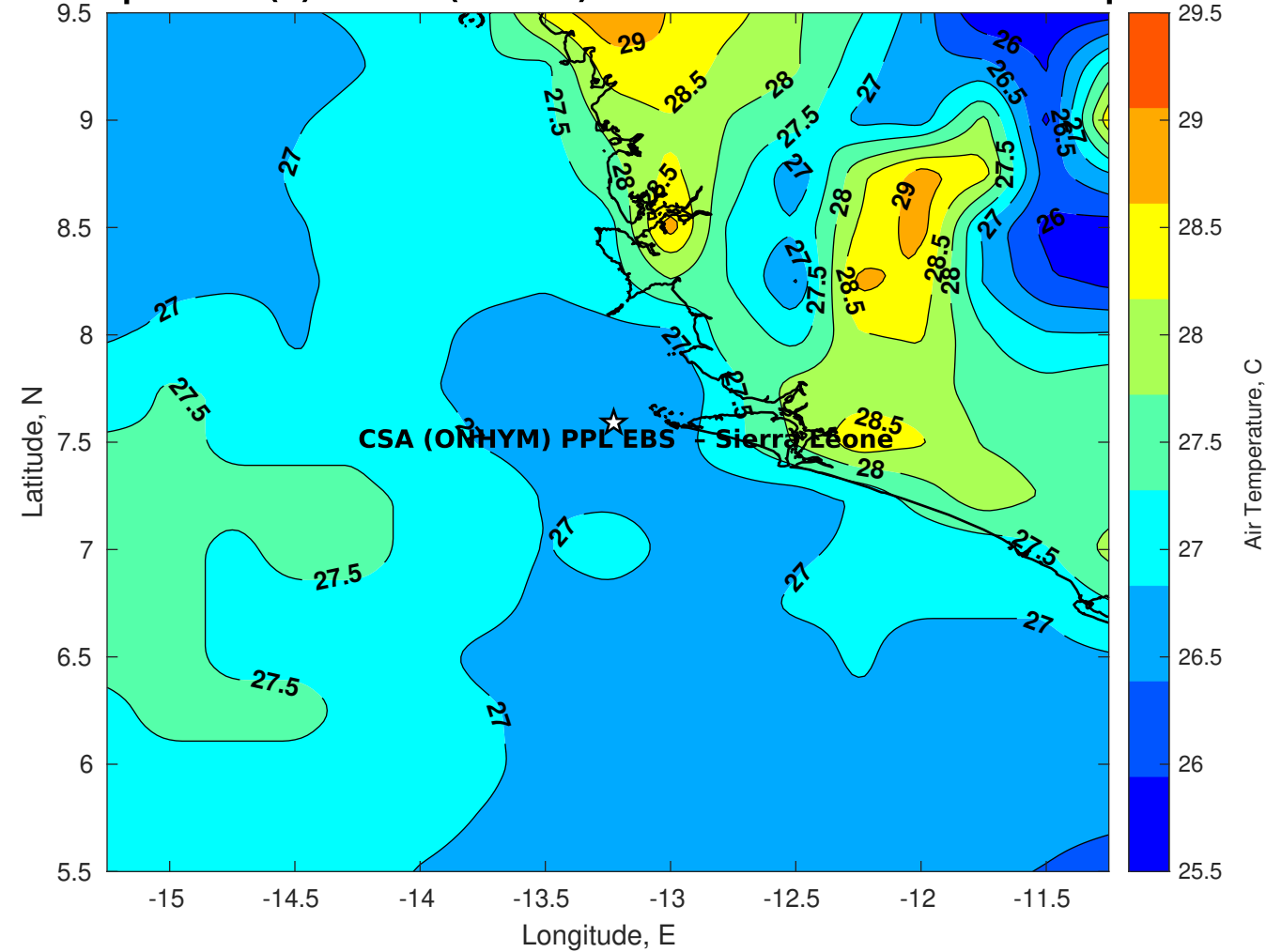
Air Temperature (C) for CSA (ONHYM) PPL EBS - Sierra Leone at 09-Sep-2025
