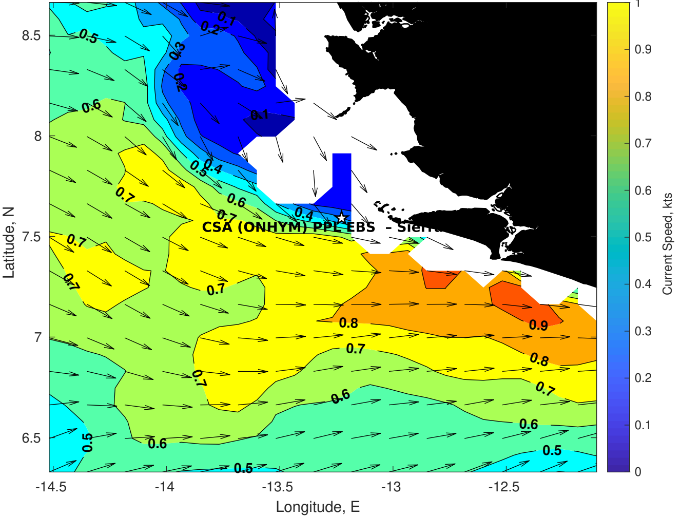
Surface Currents for CSA (ONHYM) PPL EBS - Sierra Leone at 09-Sep-2025 00:00:00
