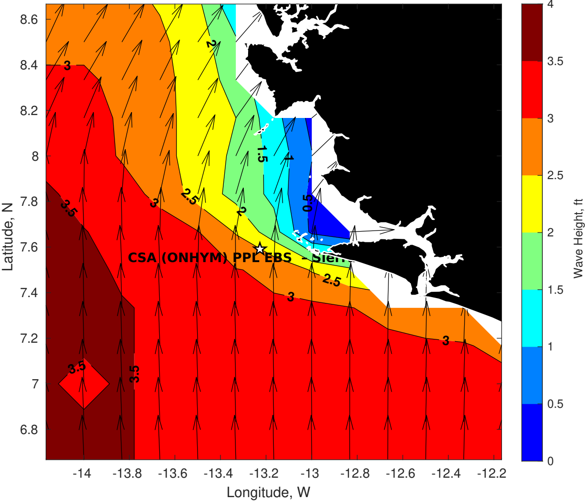
Wave Height (ft) for CSA (ONHYM) PPL EBS - Sierra Leone at 10-Sep-2025 09:00:00
