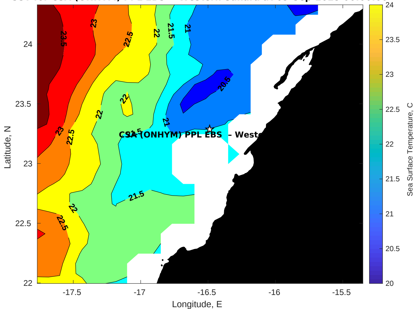
SST for CSA (ONHYM) PPL EBS - Western Sahara at 09-Sep-2025 00:00:00
