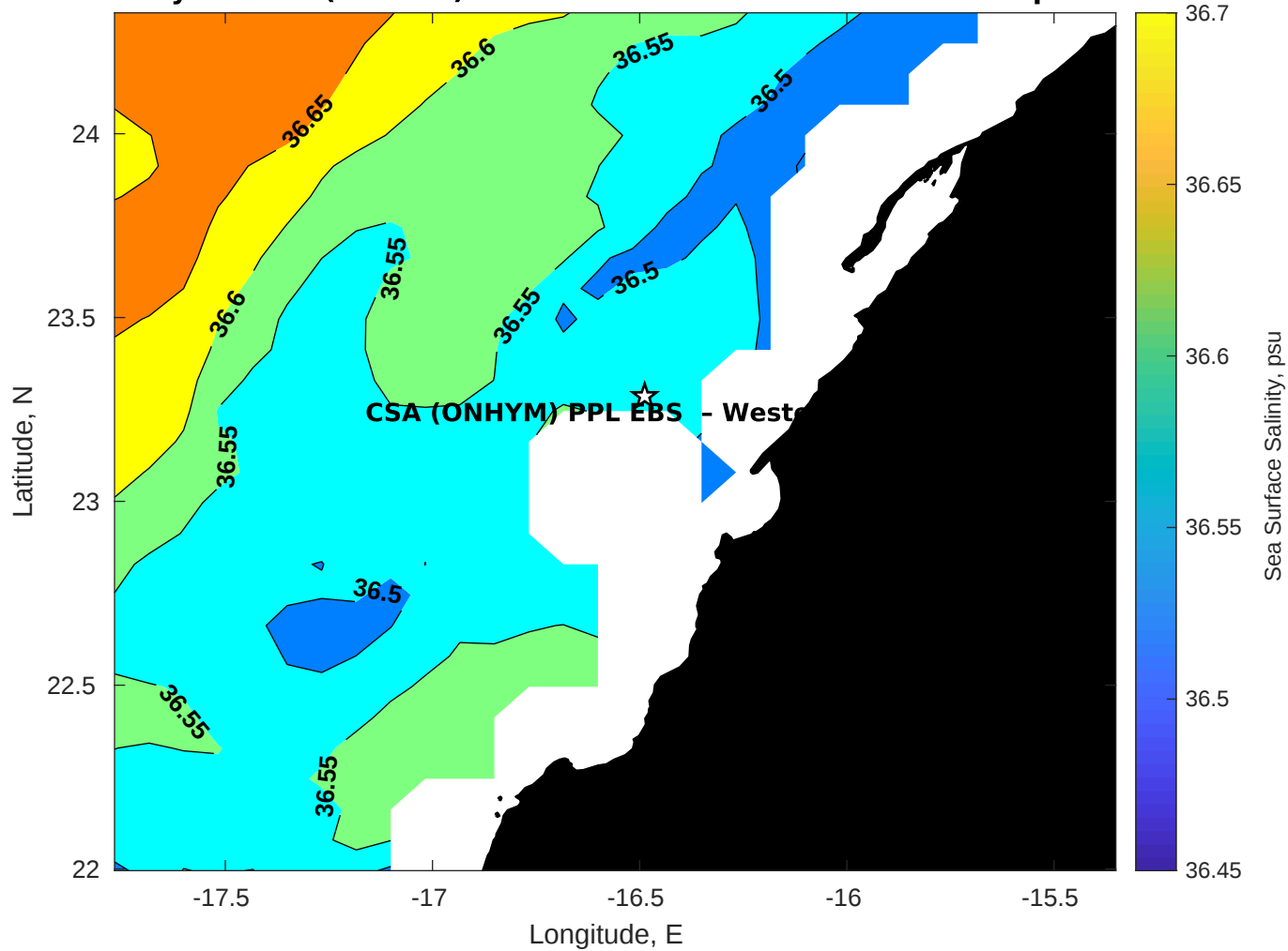
Surface Salinity for CSA (ONHYM) PPL EBS - Western Sahara at 09-Sep-2025 00:00:00
