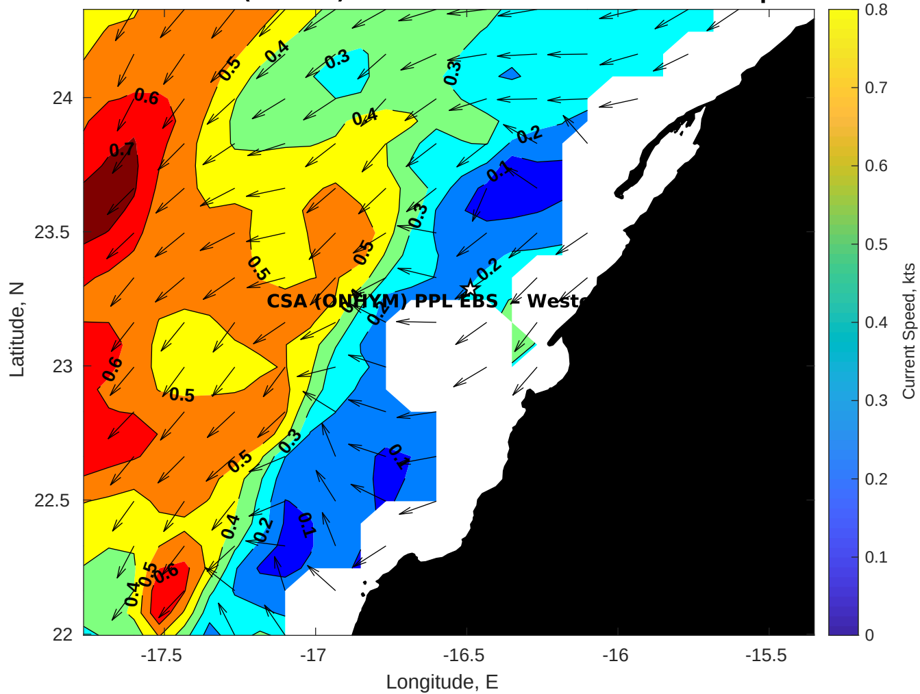
Surface Currents for CSA (ONHYM) PPL EBS - Western Sahara at 09-Sep-2025 00:00:00
