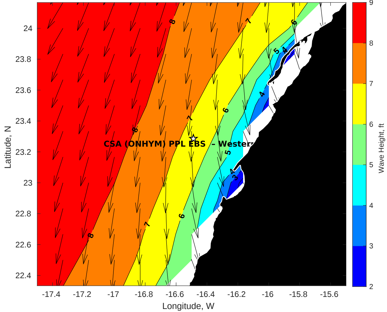
Wave Height (ft) for CSA (ONHYM) PPL EBS - Western Sahara at 10-Sep-2025 09:00:00
