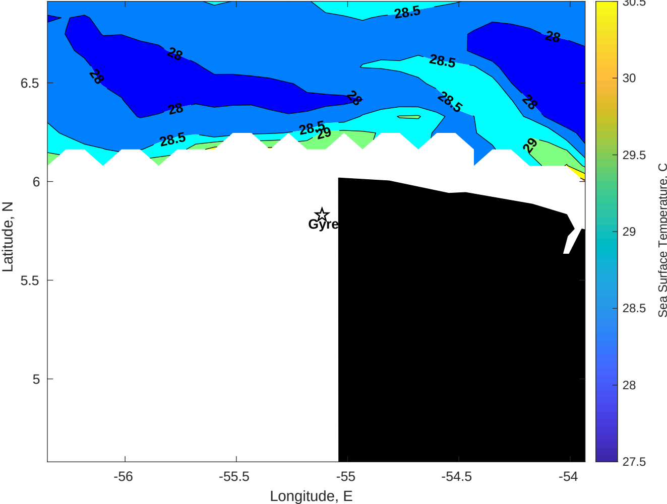
SST for Gyre at 09-Sep-2025 00:00:00
