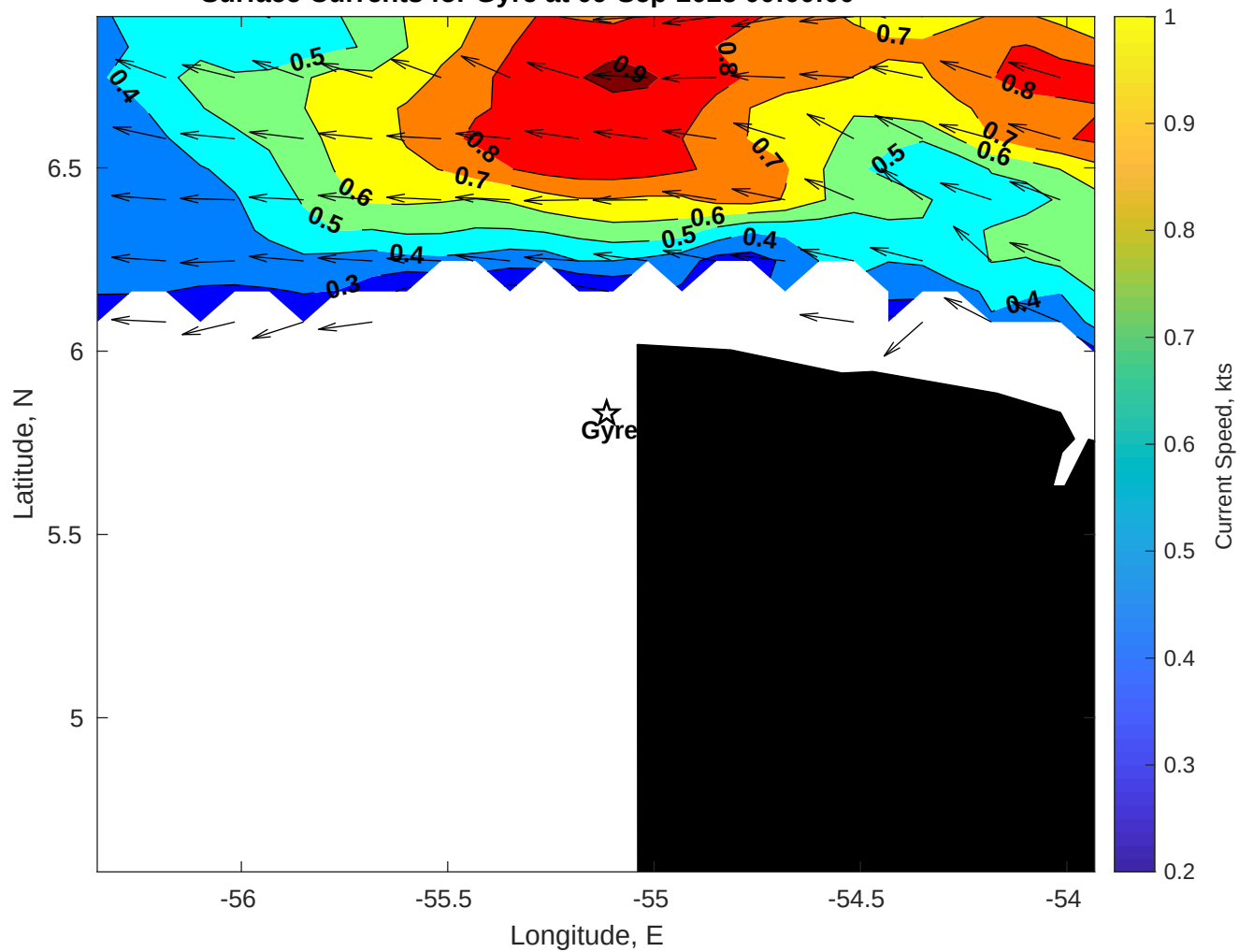
Surface Currents for Gyre at 09-Sep-2025 00:00:00
