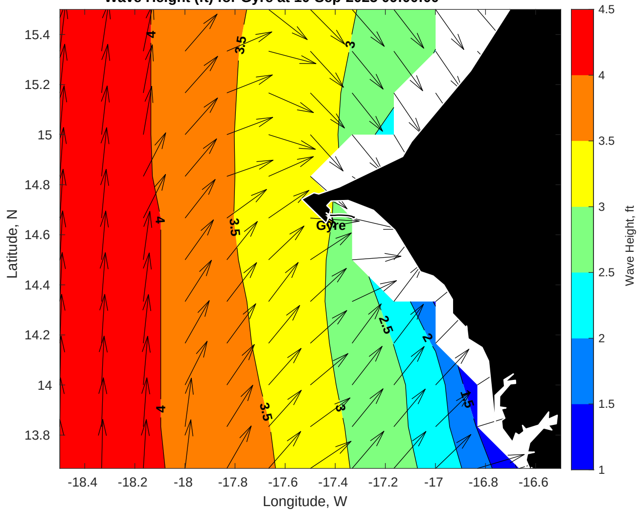
Wave Height (ft) for Gyre at 10-Sep-2025 09:00:00
