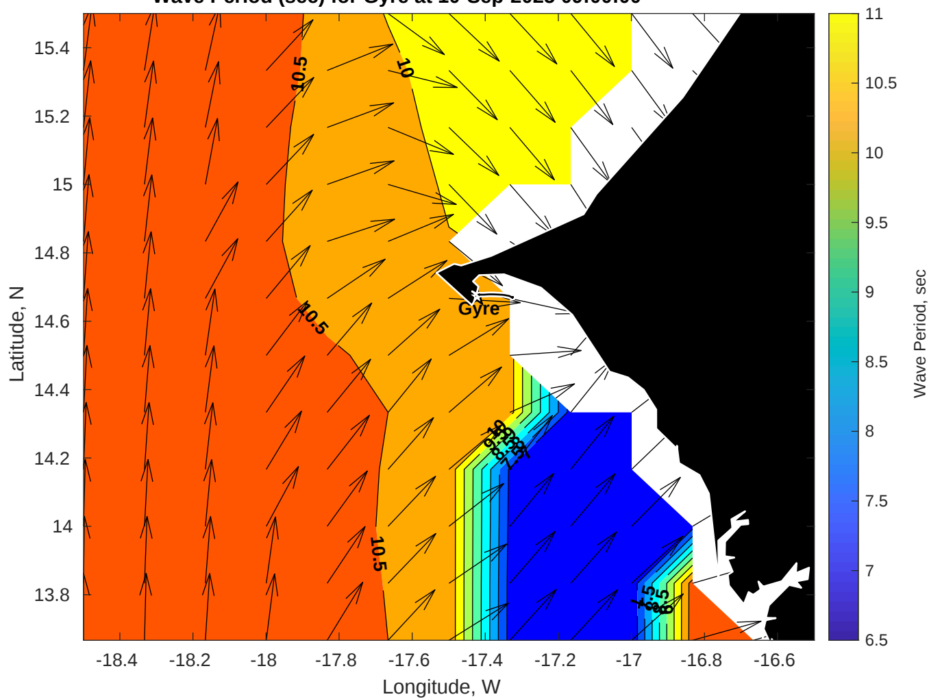
Wave Period (sec) for Gyre at 10-Sep-2025 09:00:00
