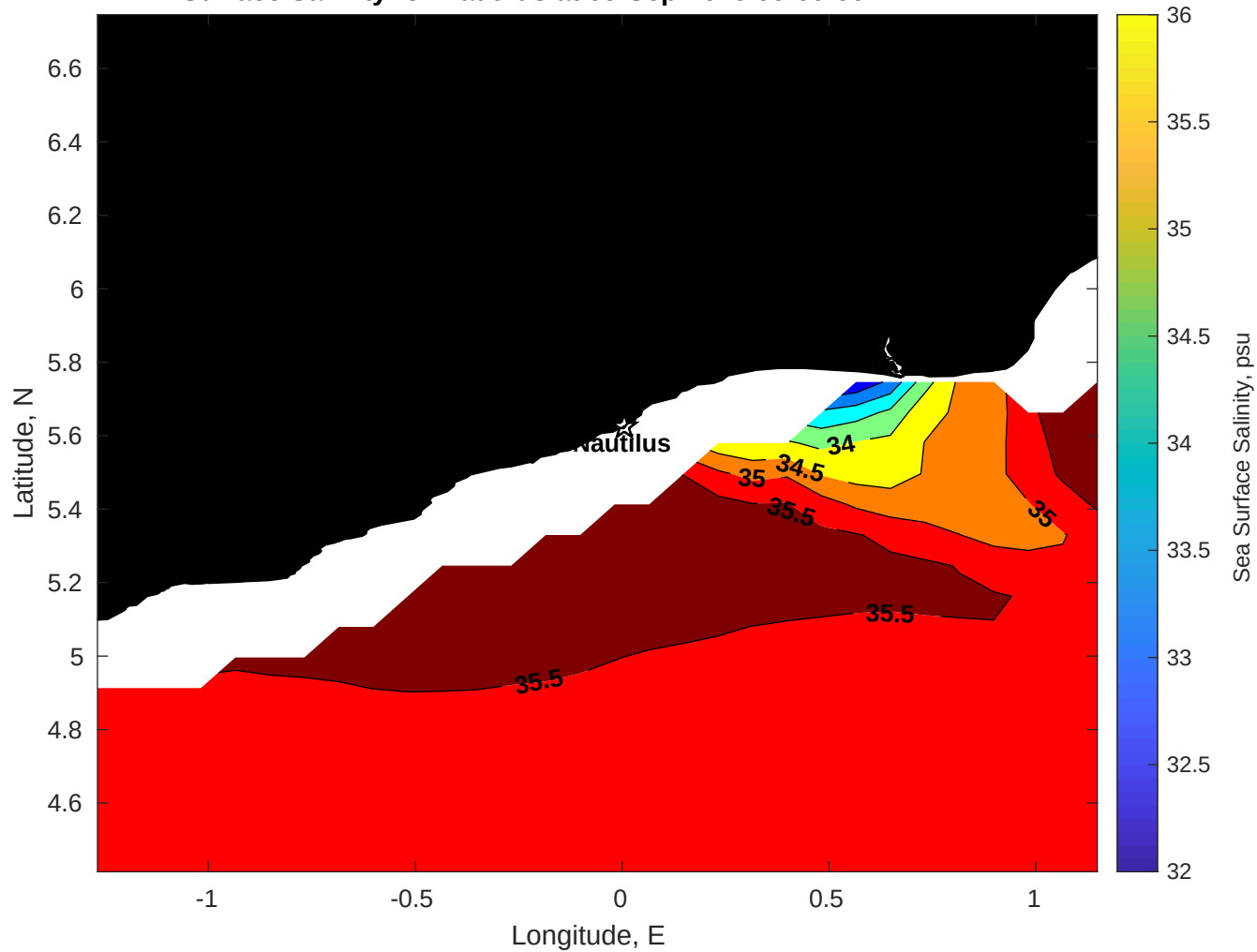
Surface Salinity for Nautilus at 09-Sep-2025 00:00:00
