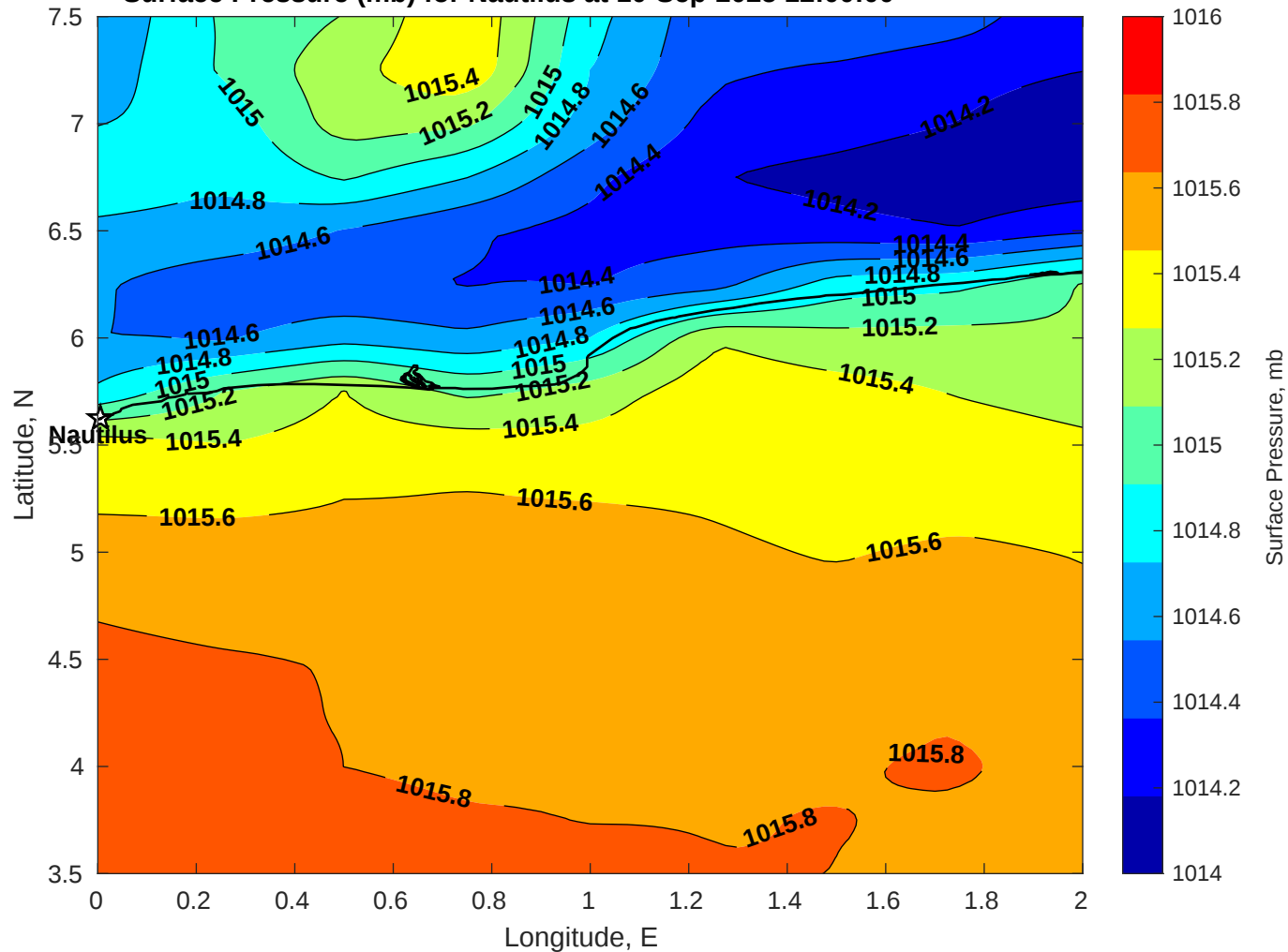
Surface Pressure (mb) for Nautilus at 10-Sep-2025 12:00:00
