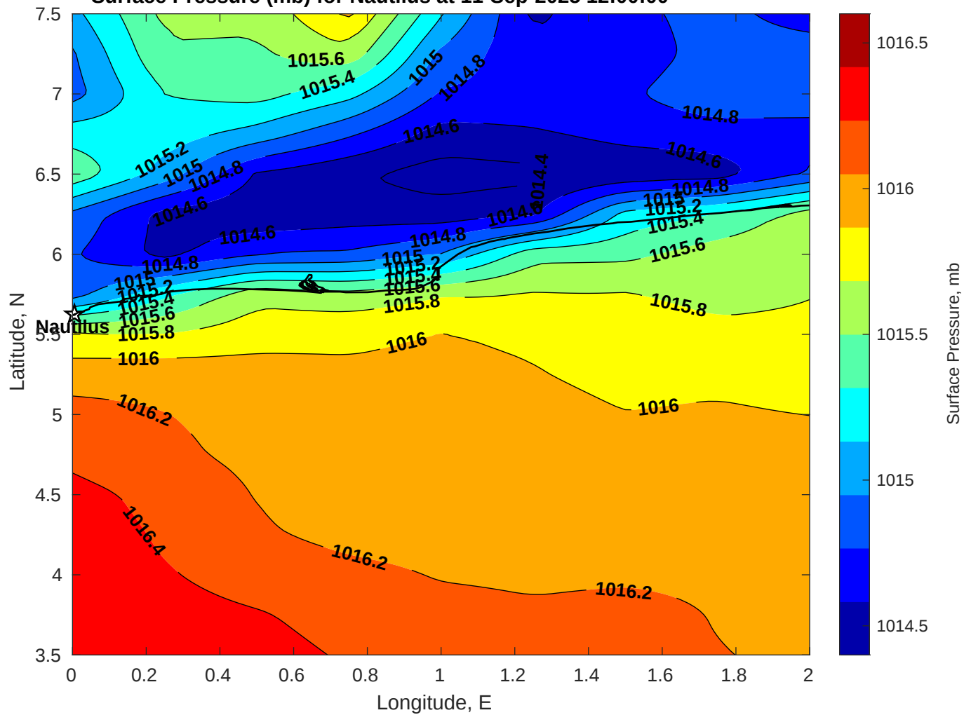
Surface Pressure (mb) for Nautilus at 11-Sep-2025 12:00:00
