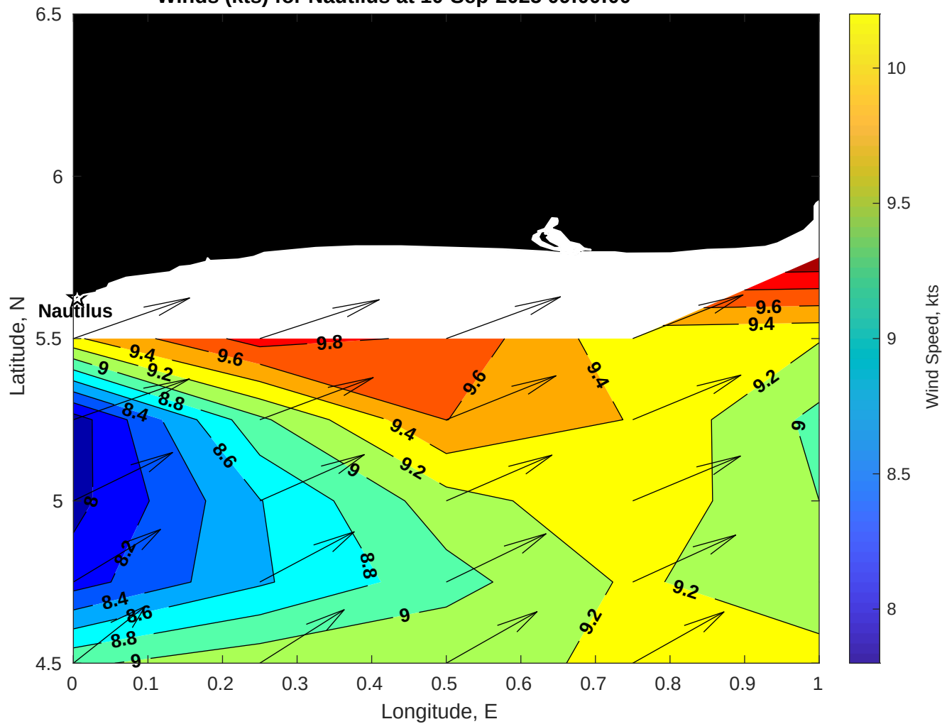
Winds (kts) for Nautilus at 10-Sep-2025 09:00:00
