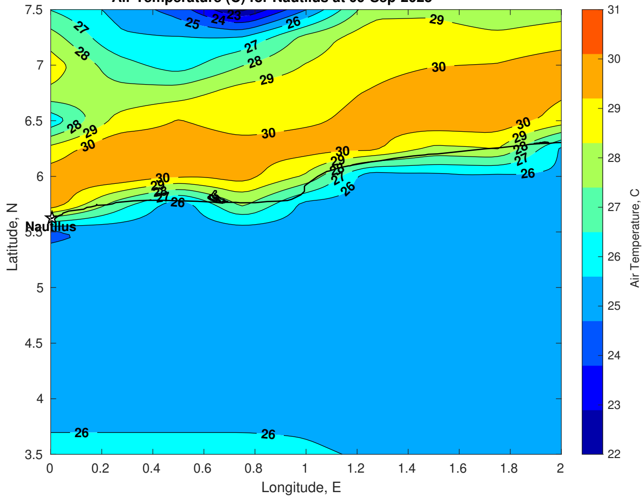
Air Temperature (C) for Nautilus at 09-Sep-2025
