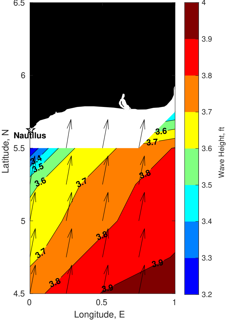
Wave Height (ft) for Nautilus at 10-Sep-2025 09:00:00
