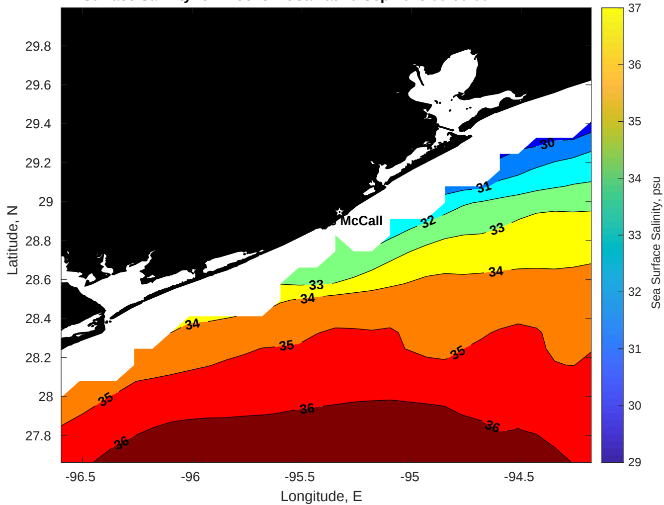
Surface Salinity for Brooks McCall at 10-Sep-2025 00:00:00
