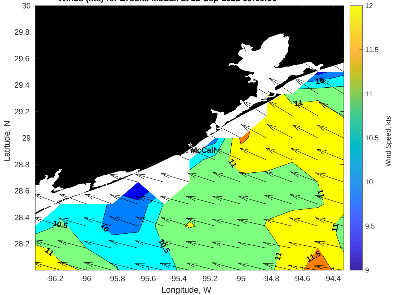
Winds (kts) for Brooks McCall at 11-Sep-2025 09:00:00
