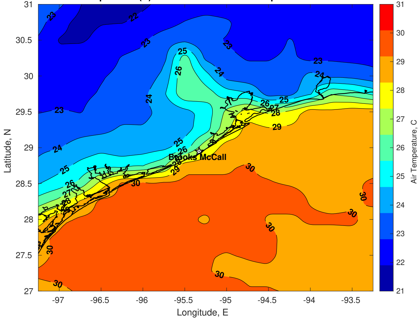
Air Temperature (C) for Brooks McCall at 10-Sep-2025
