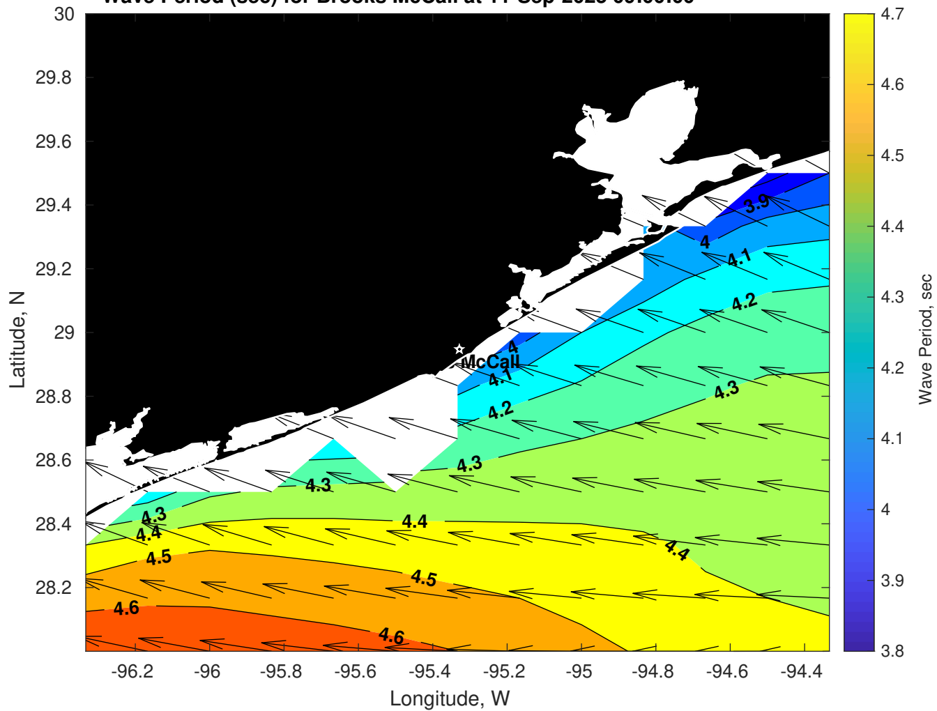
Wave Period (sec) for Brooks McCall at 11-Sep-2025 09:00:00
