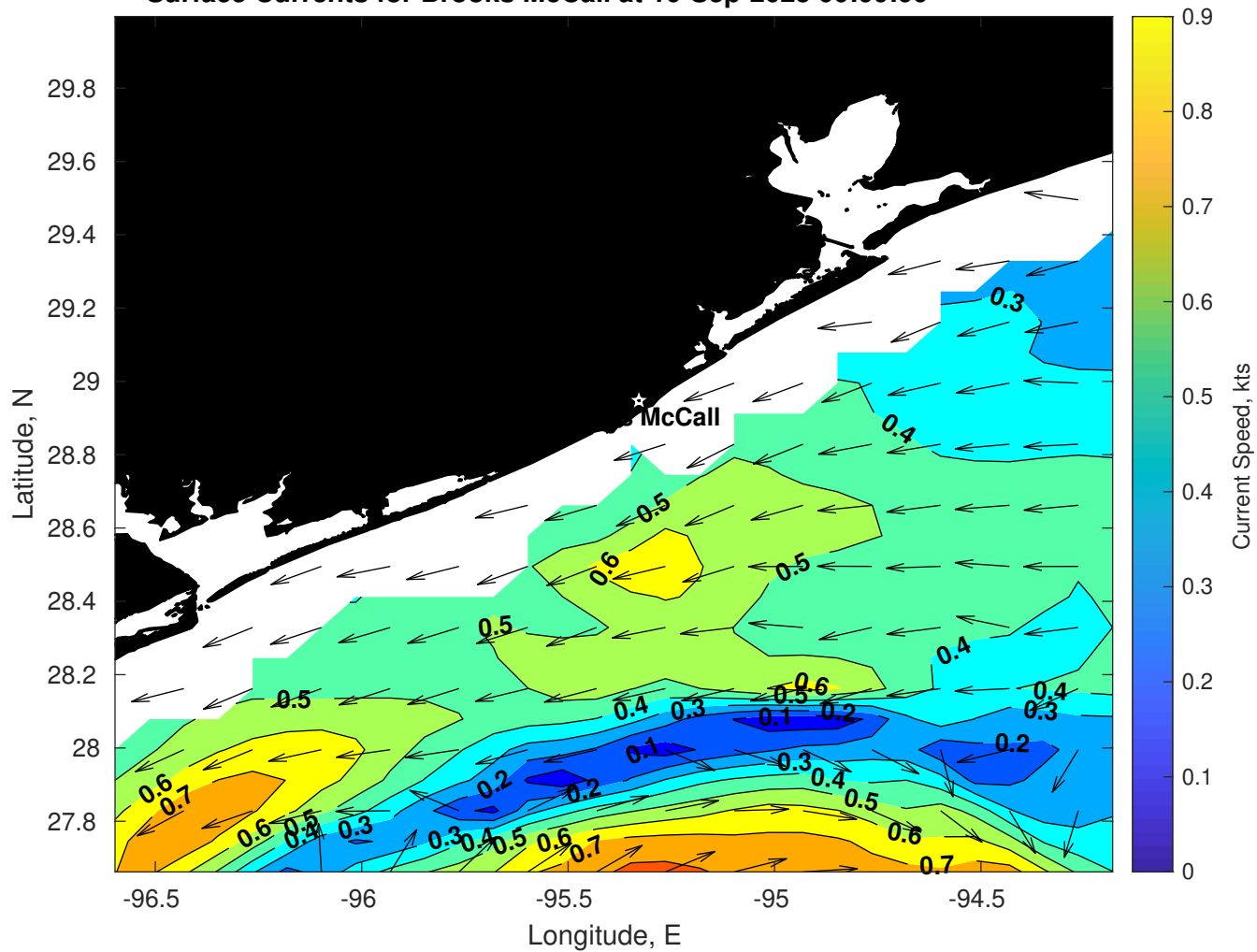
Surface Currents for Brooks McCall at 10-Sep-2025 00:00:00
