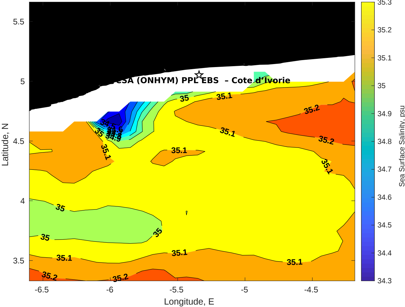
Surface Salinity for CSA (ONHYM) PPL EBS - Cote d'Ivoire at 10-Sep-2025 00:00:00
