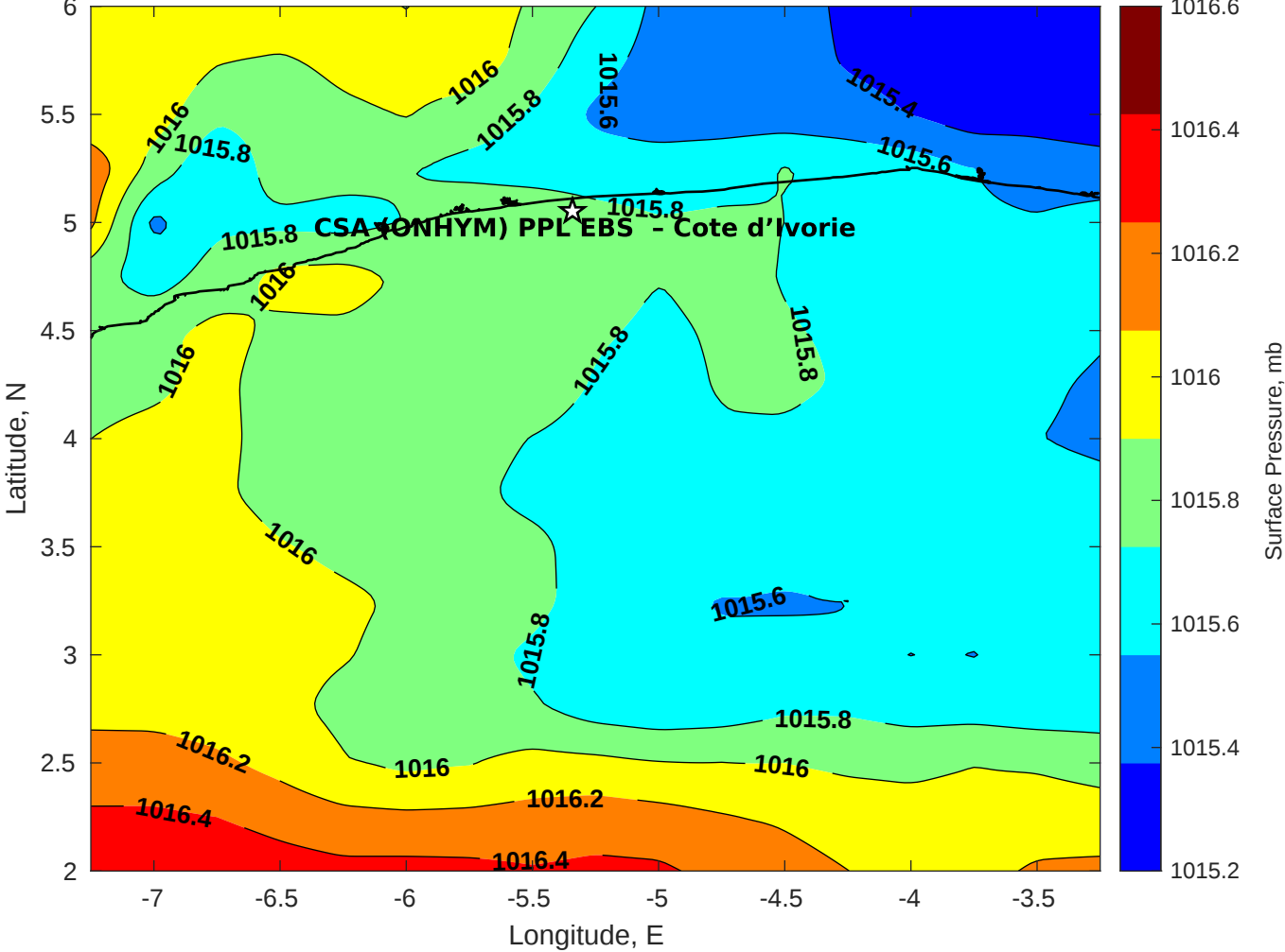
Surface Pressure (mb) for CSA (ONHYM) PPL EBS - Cote d'Ivoire at 12-Sep-2025 12:00:00
