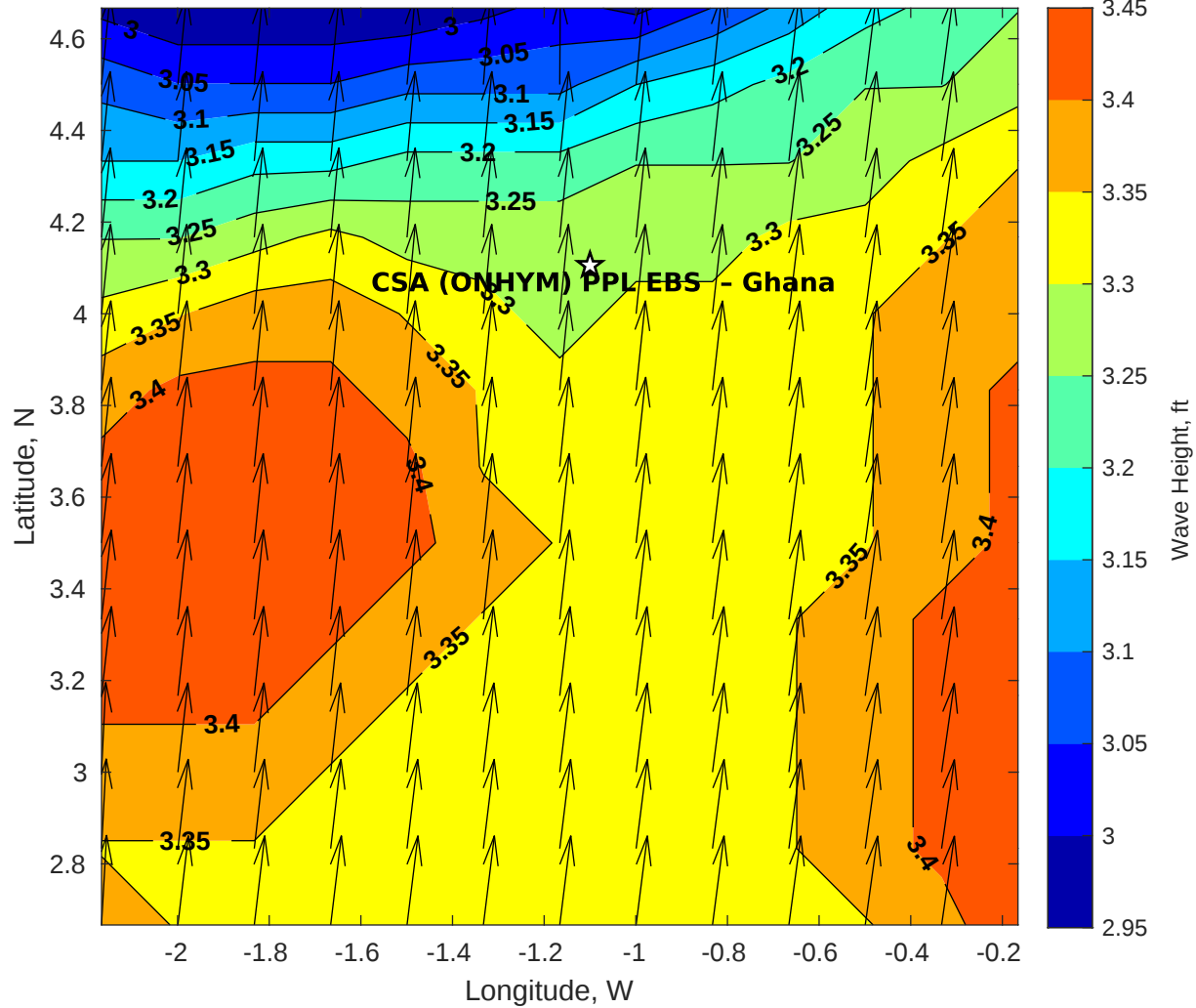
Wave Height (ft) for CSA (ONHYM) PPL EBS - Ghana at 11-Sep-2025 09:00:00
