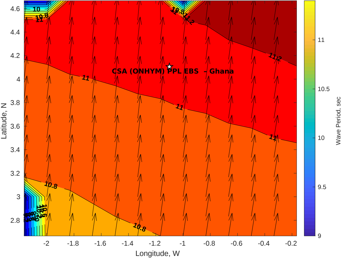
Wave Period (sec) for CSA (ONHYM) PPL EBS - Ghana at 11-Sep-2025 09:00:00
