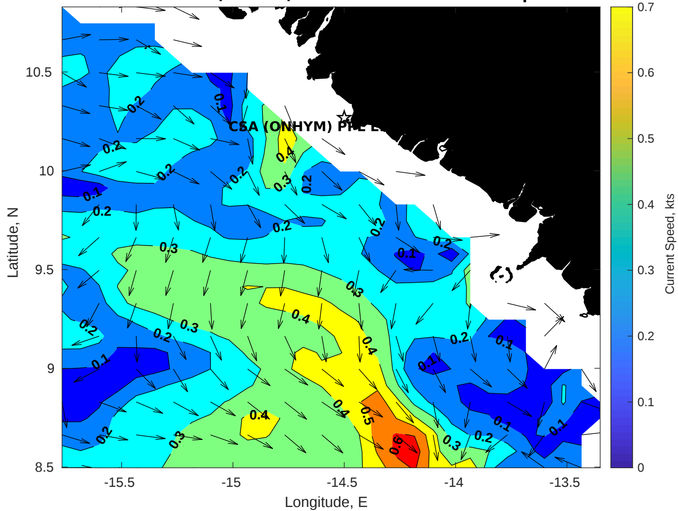
Surface Currents for CSA (ONHYM) PPL EBS - Guinea at 10-Sep-2025 00:00:00
