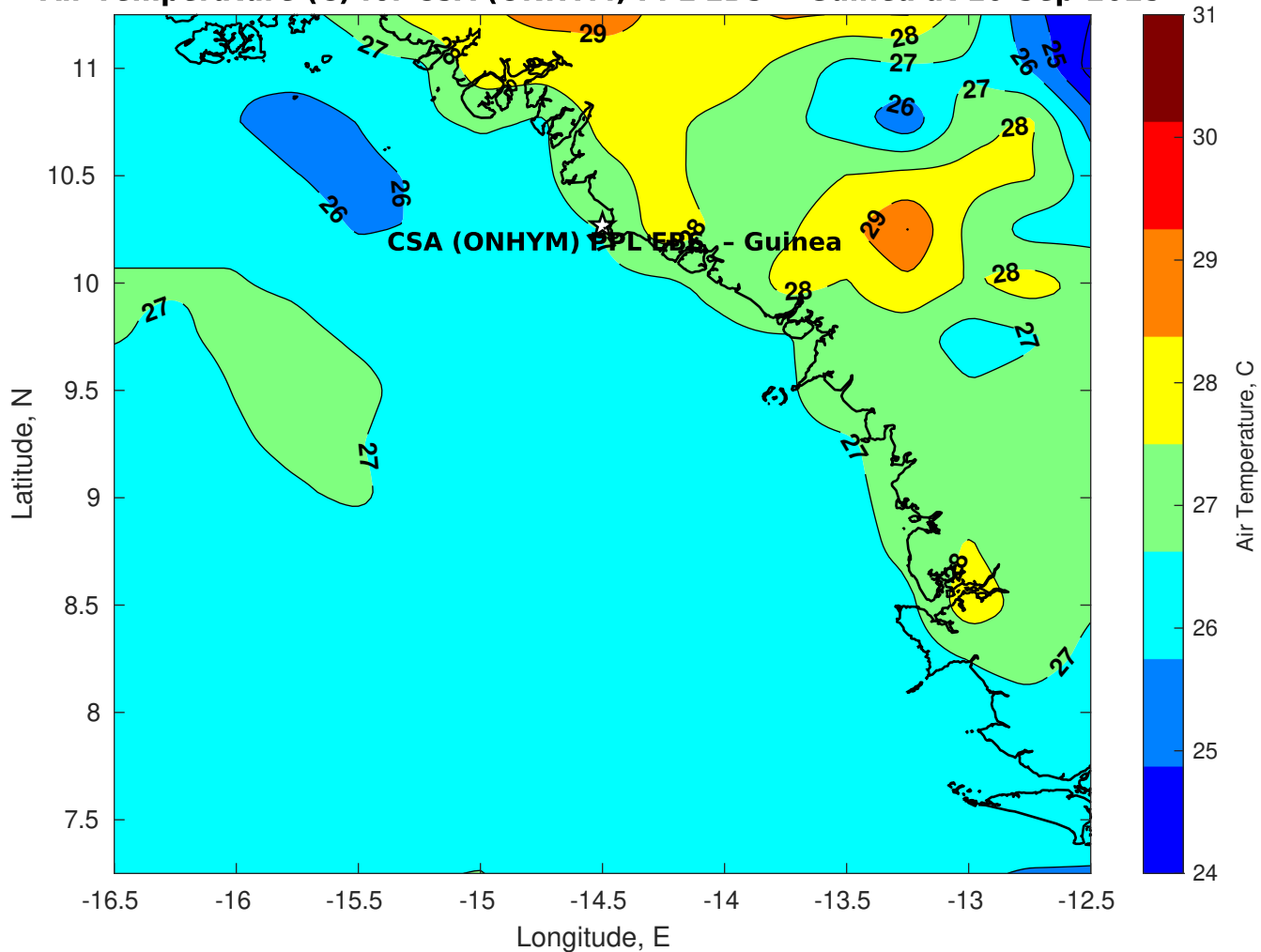
Air Temperature (C) for CSA (ONHYM) PPL EBS - Guinea at 10-Sep-2025
