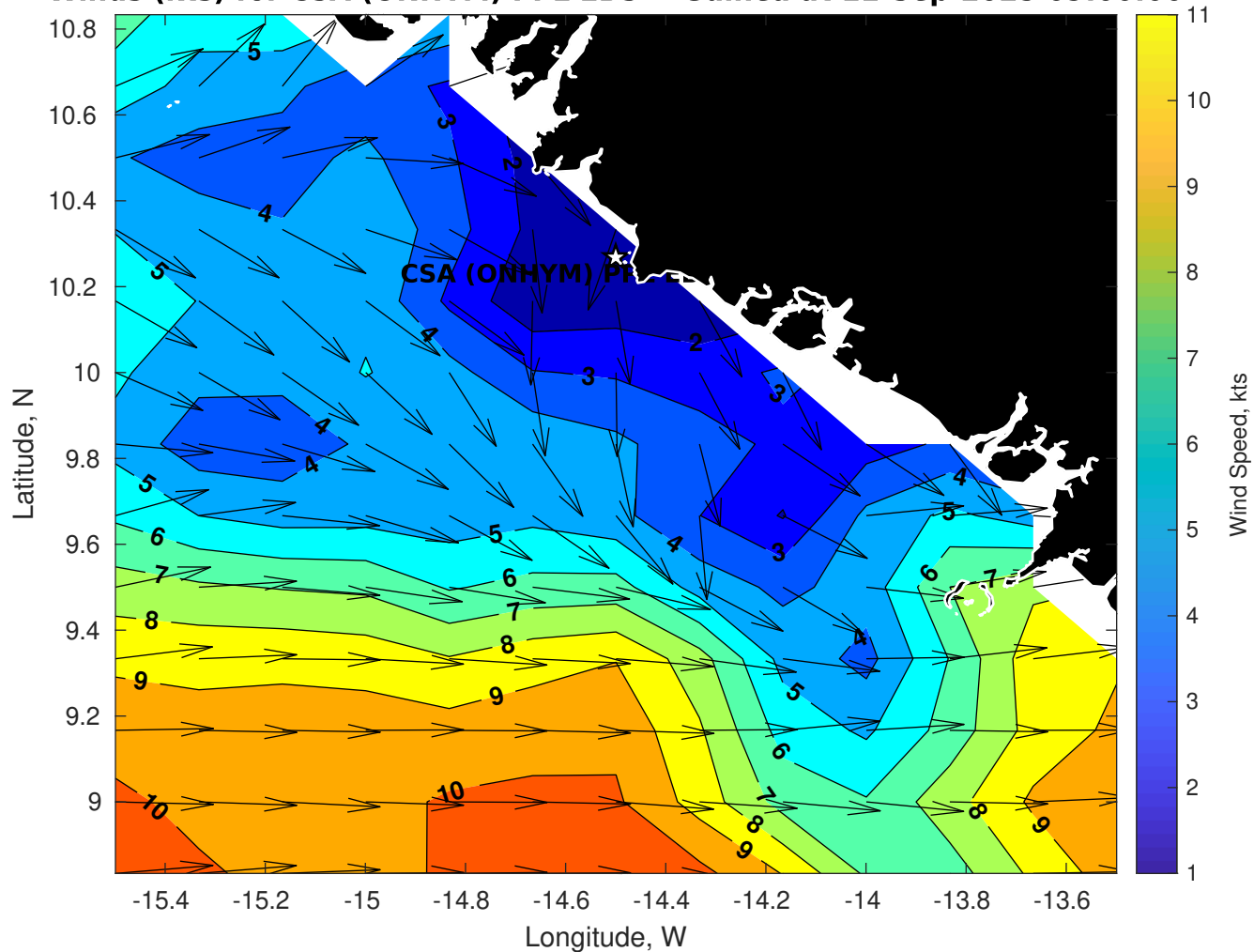
Winds (kts) for CSA (ONHYM) PPL EBS - Guinea at 11-Sep-2025 09:00:00
