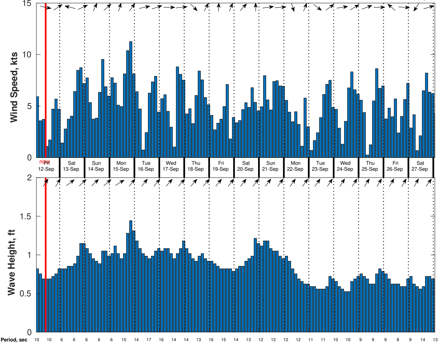
Wind & Wave Forecast for CSA (ONHYM) PPL EBS - Guinea from 11-Sep-2025 01:00:00 to 27-Sep-2025 01:00:00
