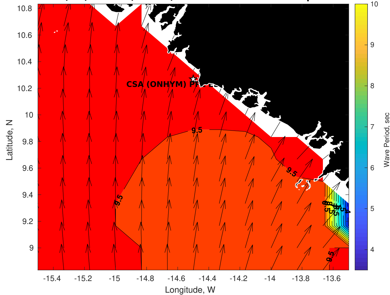
Wave Period (sec) for CSA (ONHYM) PPL EBS - Guinea at 11-Sep-2025 09:00:00
