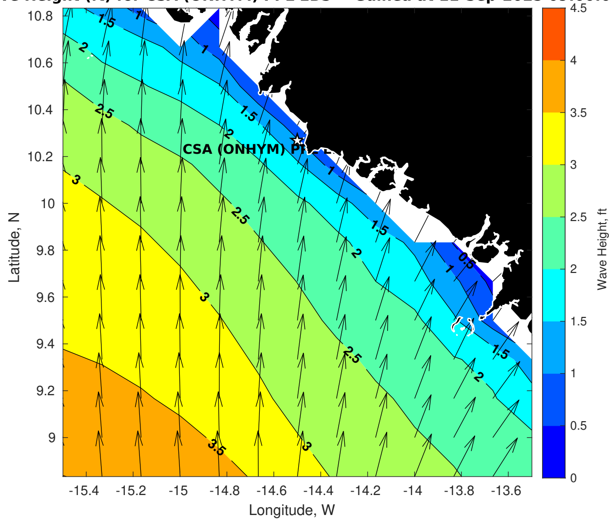
Wave Height (ft) for CSA (ONHYM) PPL EBS - Guinea at 11-Sep-2025 09:00:00
