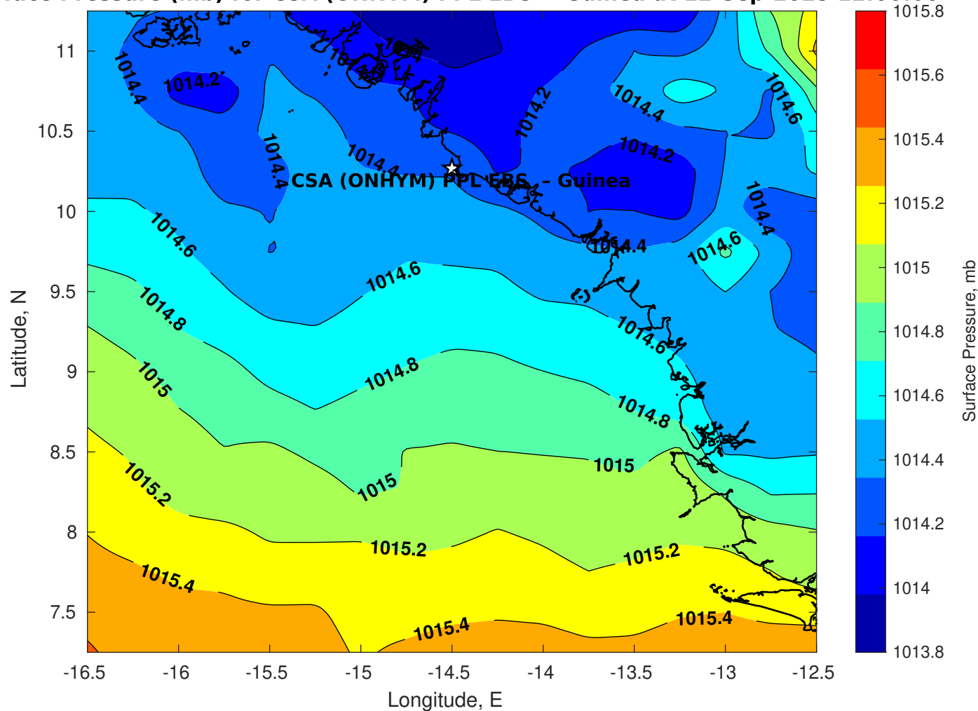
Surface Pressure (mb) for CSA (ONHYM) PPL EBS - Guinea at 12-Sep-2025 12:00:00
