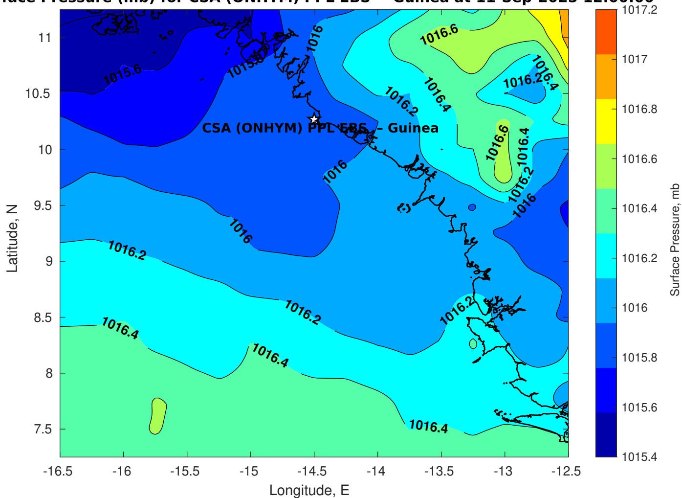
Surface Pressure (mb) for CSA (ONHYM) PPL EBS - Guinea at 11-Sep-2025 12:00:00
