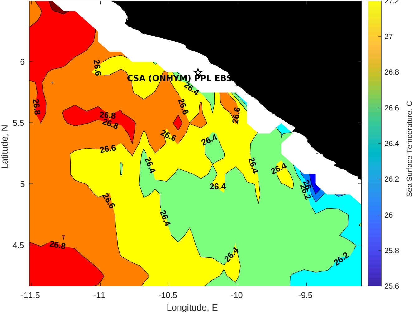
SST for CSA (ONHYM) PPL EBS - Liberia at 10-Sep-2025 00:00:00
