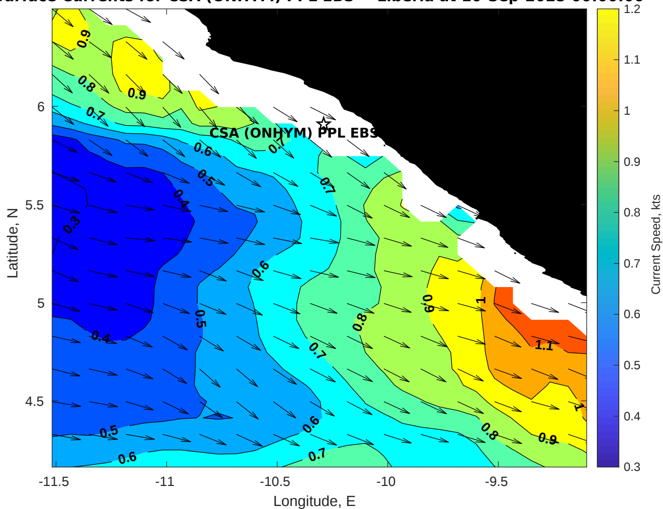
Surface Currents for CSA (ONHYM) PPL EBS - Liberia at 10-Sep-2025 00:00:00
