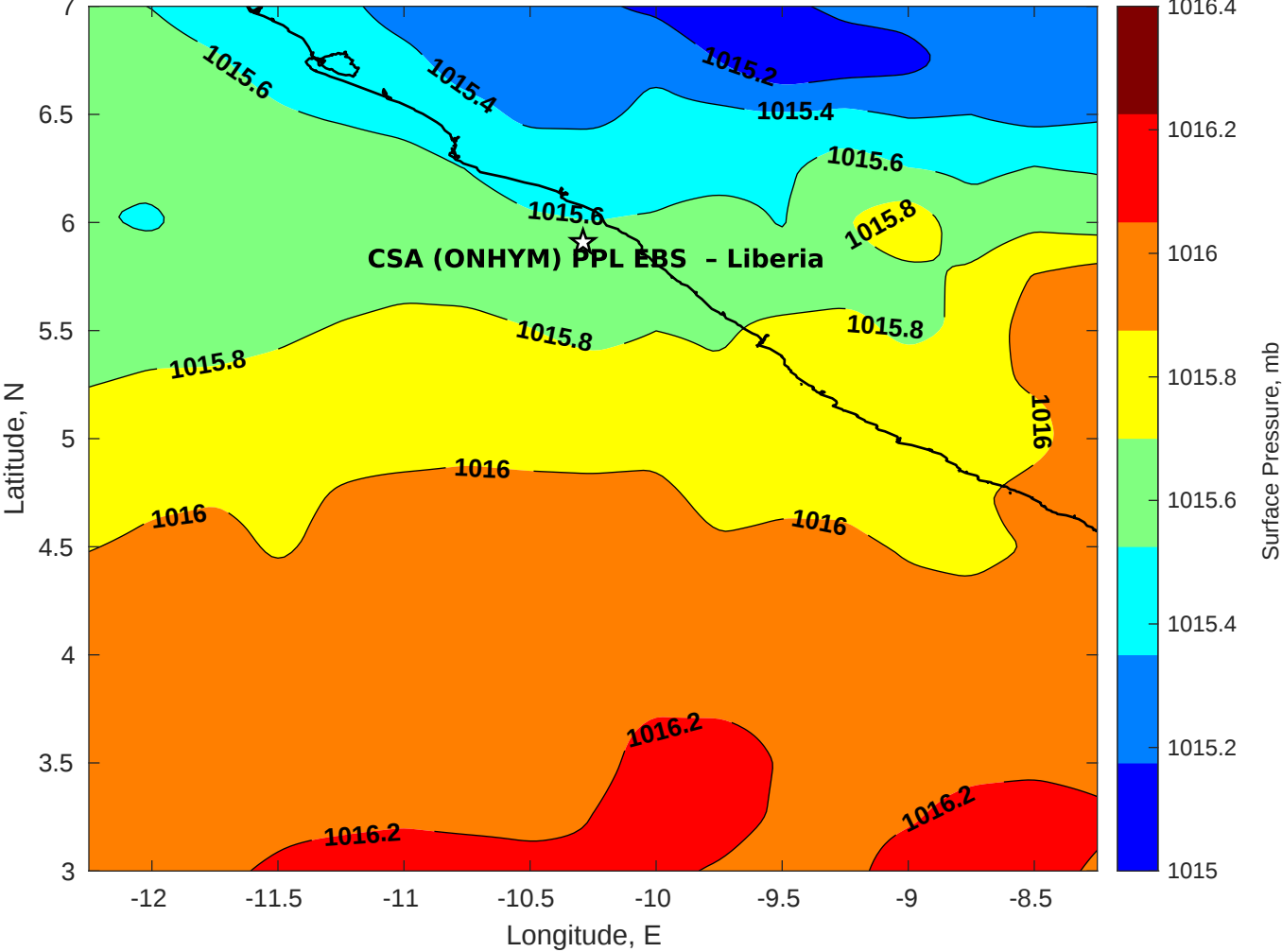
Surface Pressure (mb) for CSA (ONHYM) PPL EBS - Liberia at 12-Sep-2025 12:00:00
