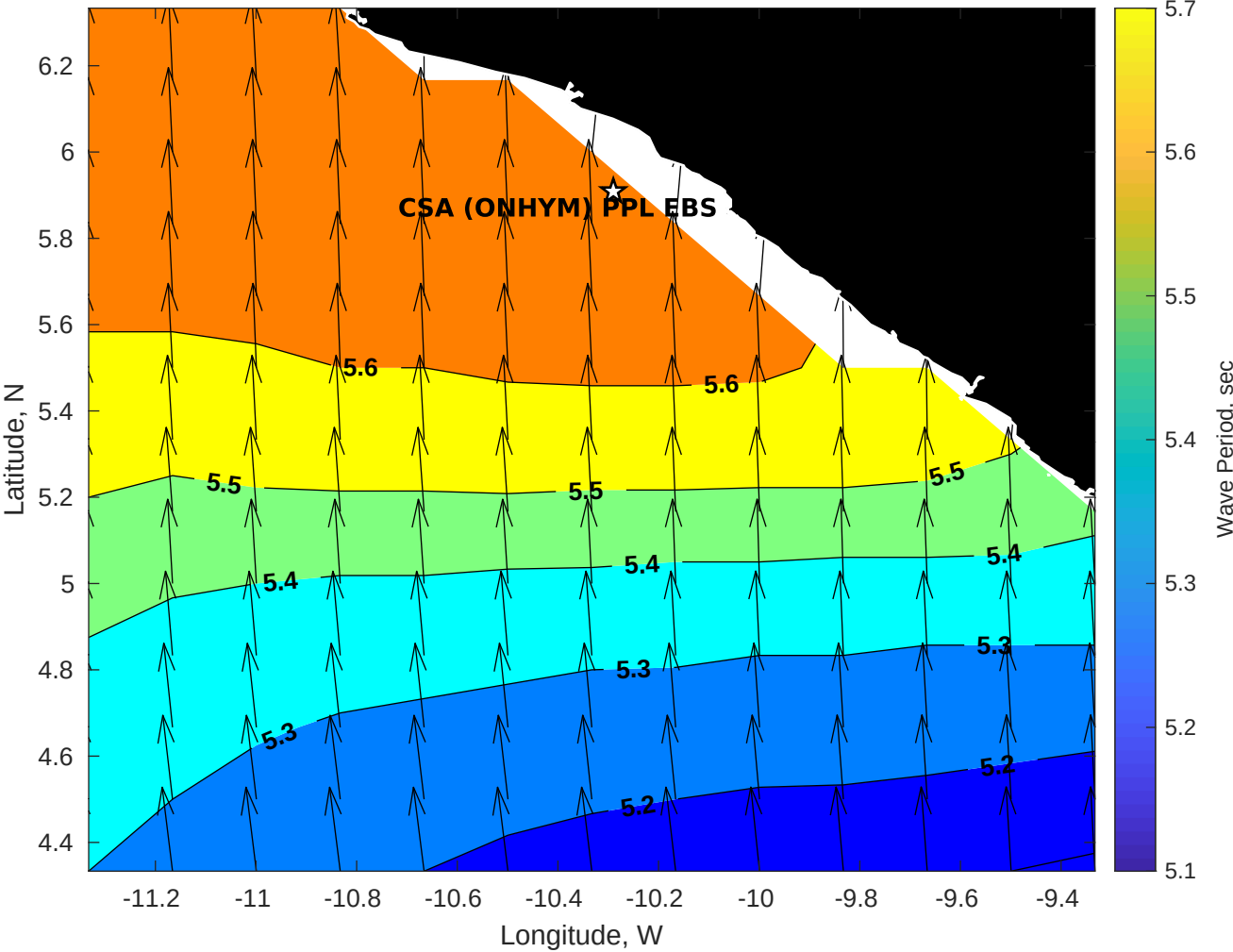
Wave Period (sec) for CSA (ONHYM) PPL EBS - Liberia at 11-Sep-2025 09:00:00
