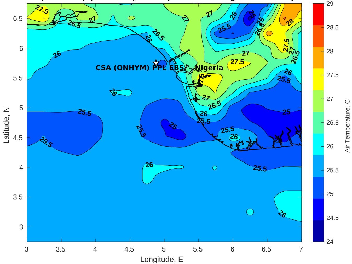
Air Temperature (C) for CSA (ONHYM) PPL EBS - Nigeria at 10-Sep-2025
