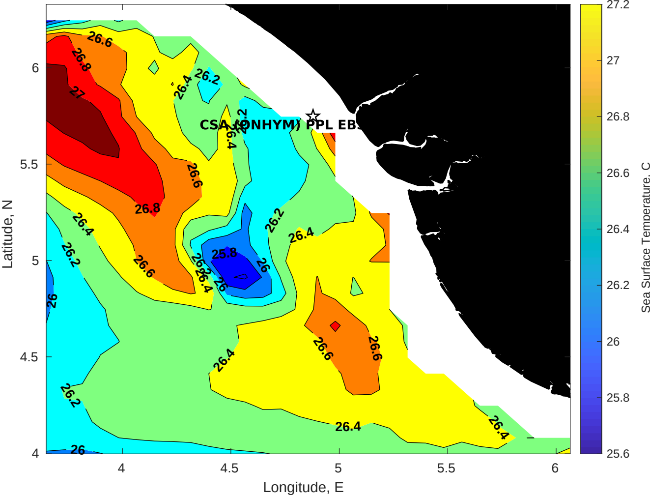
SST for CSA (ONHYM) PPL EBS - Nigeria at 10-Sep-2025 00:00:00
