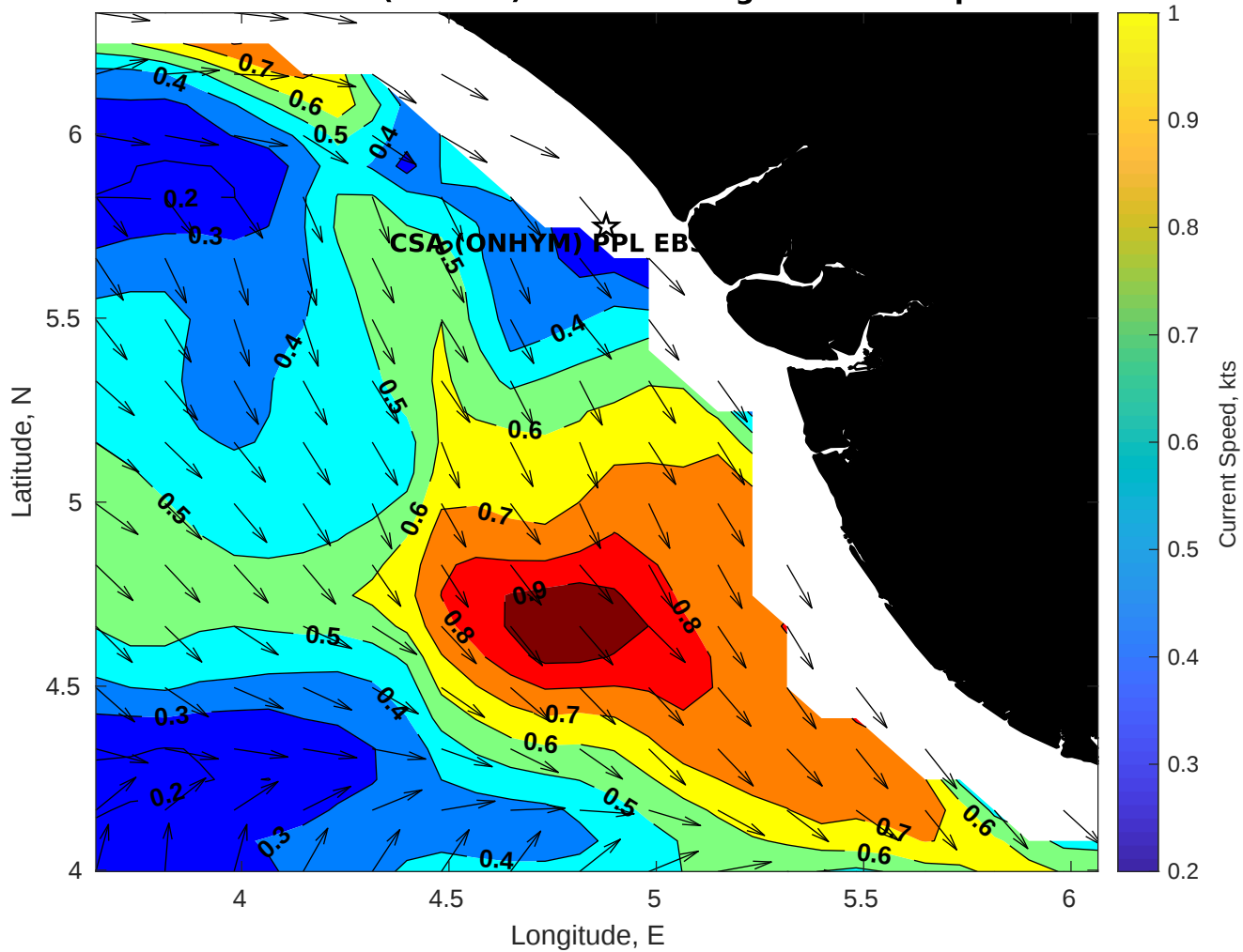
Surface Currents for CSA (ONHYM) PPL EBS - Nigeria at 10-Sep-2025 00:00:00
