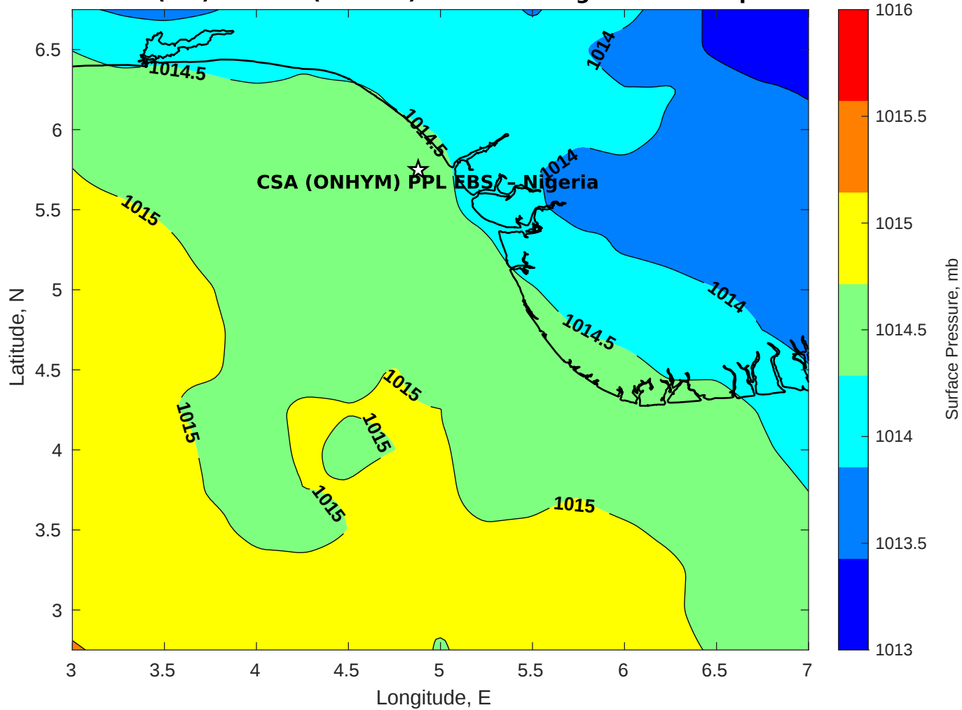
Surface Pressure (mb) for CSA (ONHYM) PPL EBS - Nigeria at 11-Sep-2025 12:00:00
