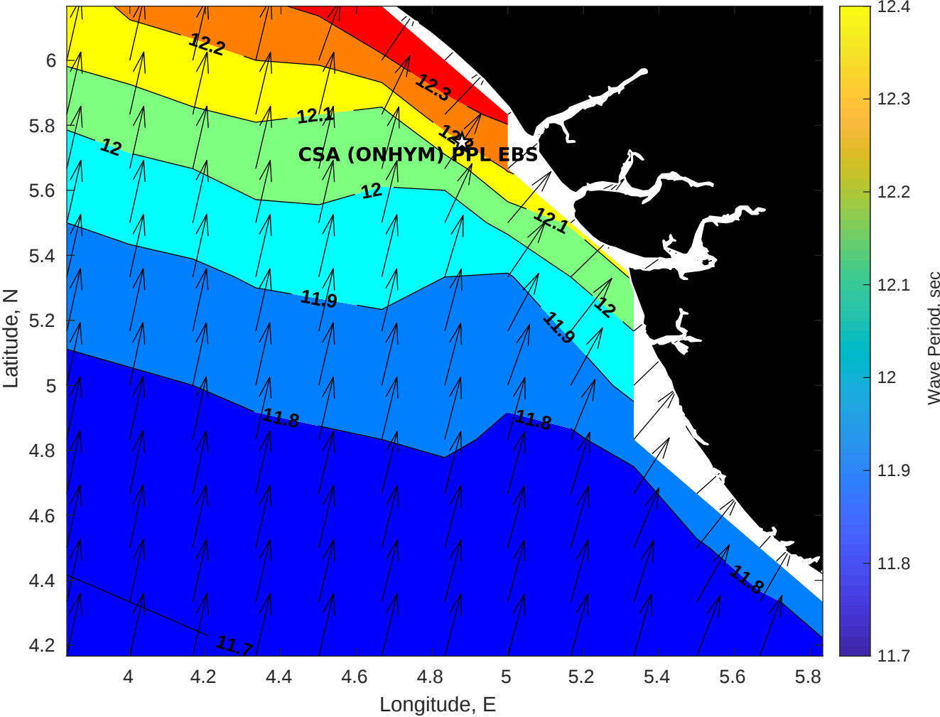
Wave Period (sec) for CSA (ONHYM) PPL EBS - Nigeria at 11-Sep-2025 09:00:00
