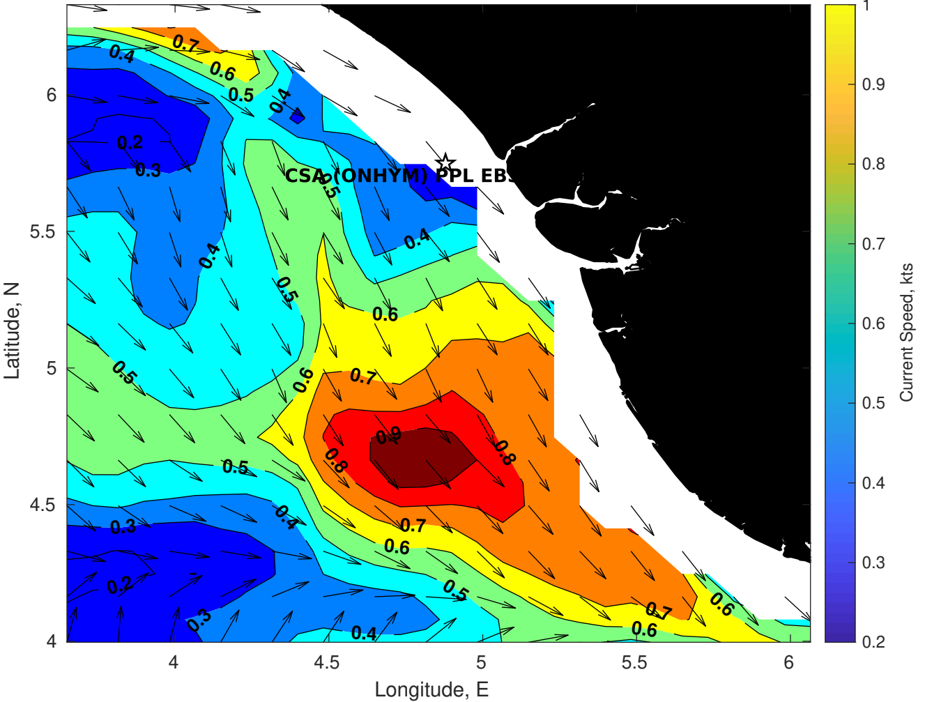
Surface Currents for CSA (ONHYM) PPL EBS - Nigeria at 10-Sep-2025 00:00:00
