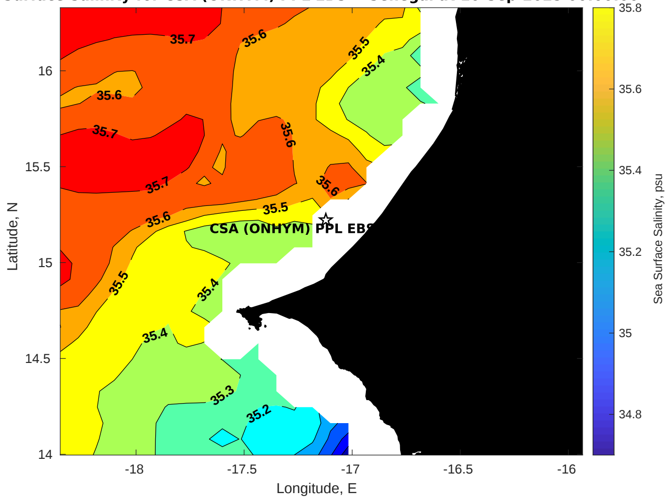
Surface Salinity for CSA (ONHYM) PPL EBS - Senegal at 10-Sep-2025 00:00:00
