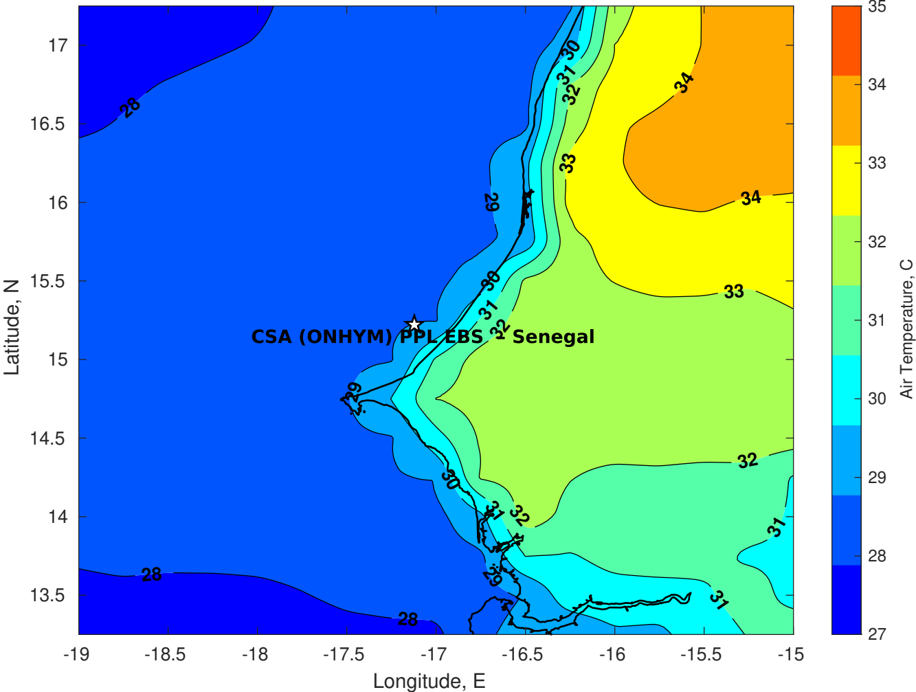
Air Temperature (C) for CSA (ONHYM) PPL EBS - Senegal at 10-Sep-2025
