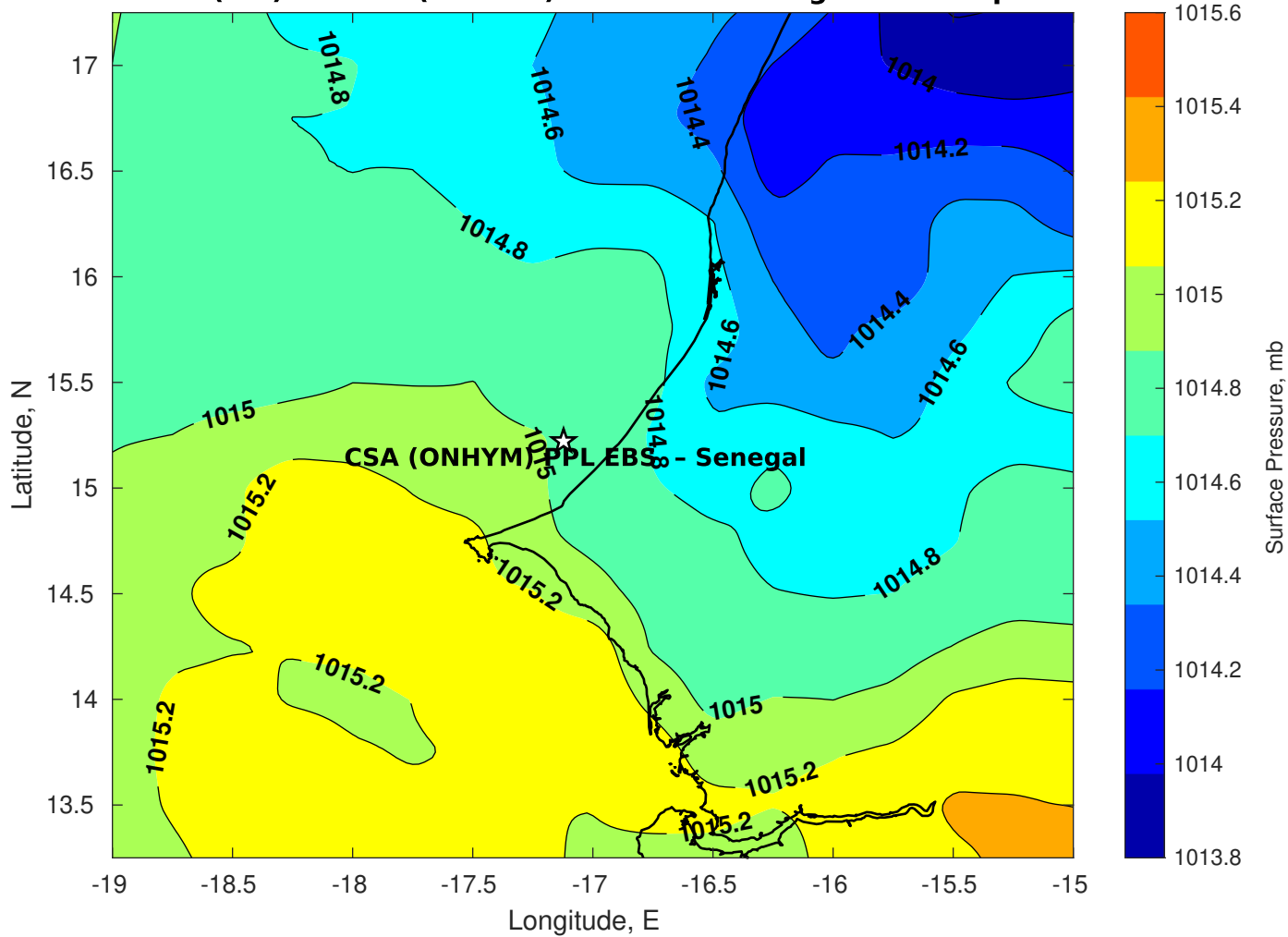
Surface Pressure (mb) for CSA (ONHYM) PPL EBS - Senegal at 11-Sep-2025 12:00:00
