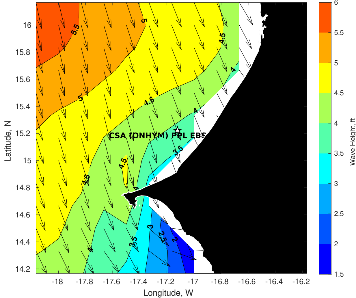
Wave Height (ft) for CSA (ONHYM) PPL EBS - Senegal at 11-Sep-2025 09:00:00
