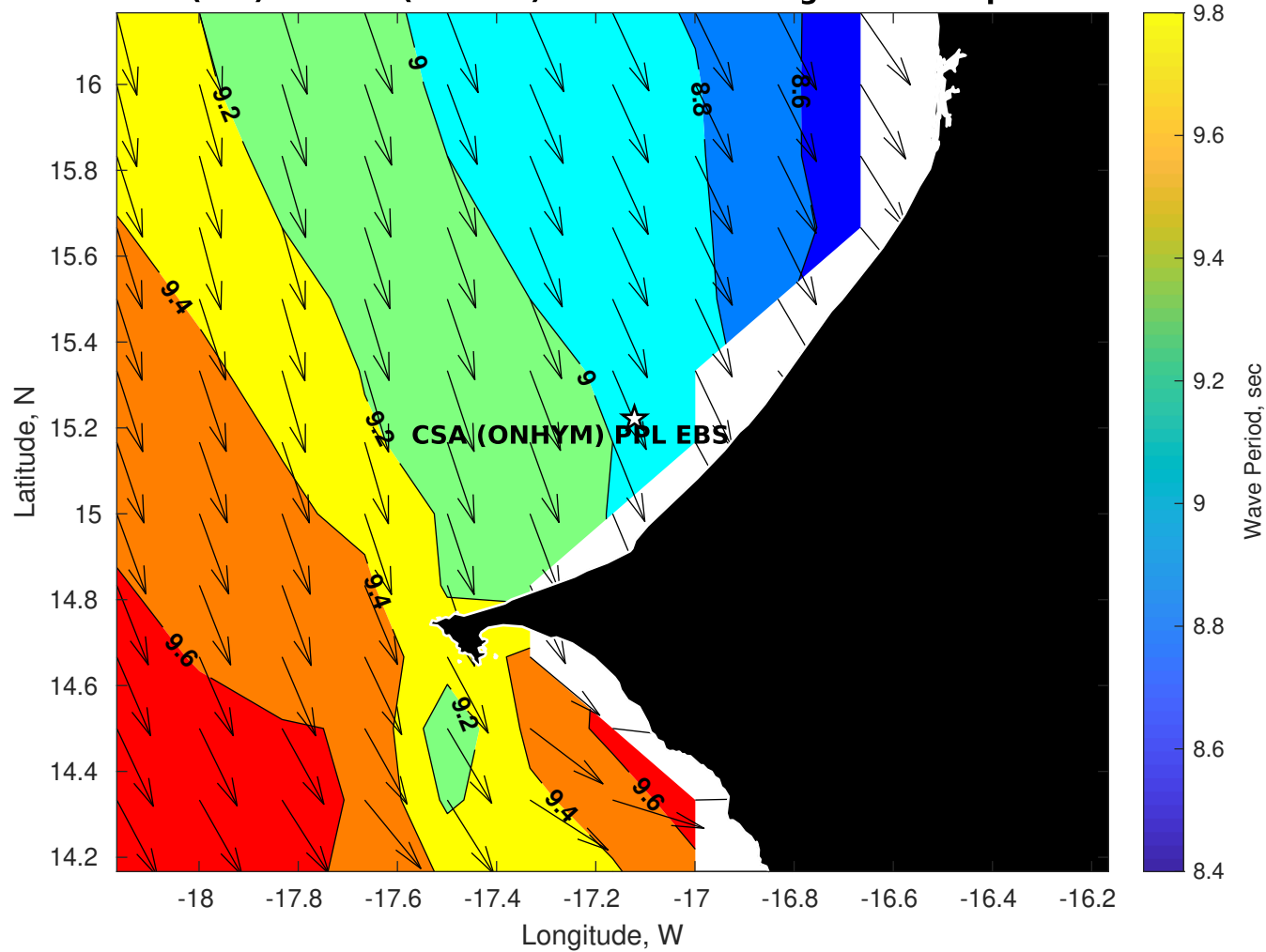
Wave Period (sec) for CSA (ONHYM) PPL EBS - Senegal at 11-Sep-2025 09:00:00
