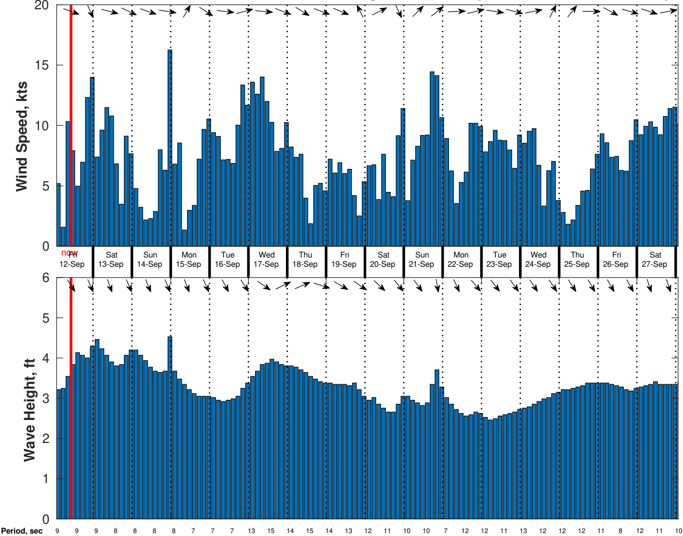
Wind & Wave Forecast for CSA (ONHYM) PPL EBS - Senegal from 11-Sep-2025 01:00:00 to 27-Sep-2025 01:00:00
