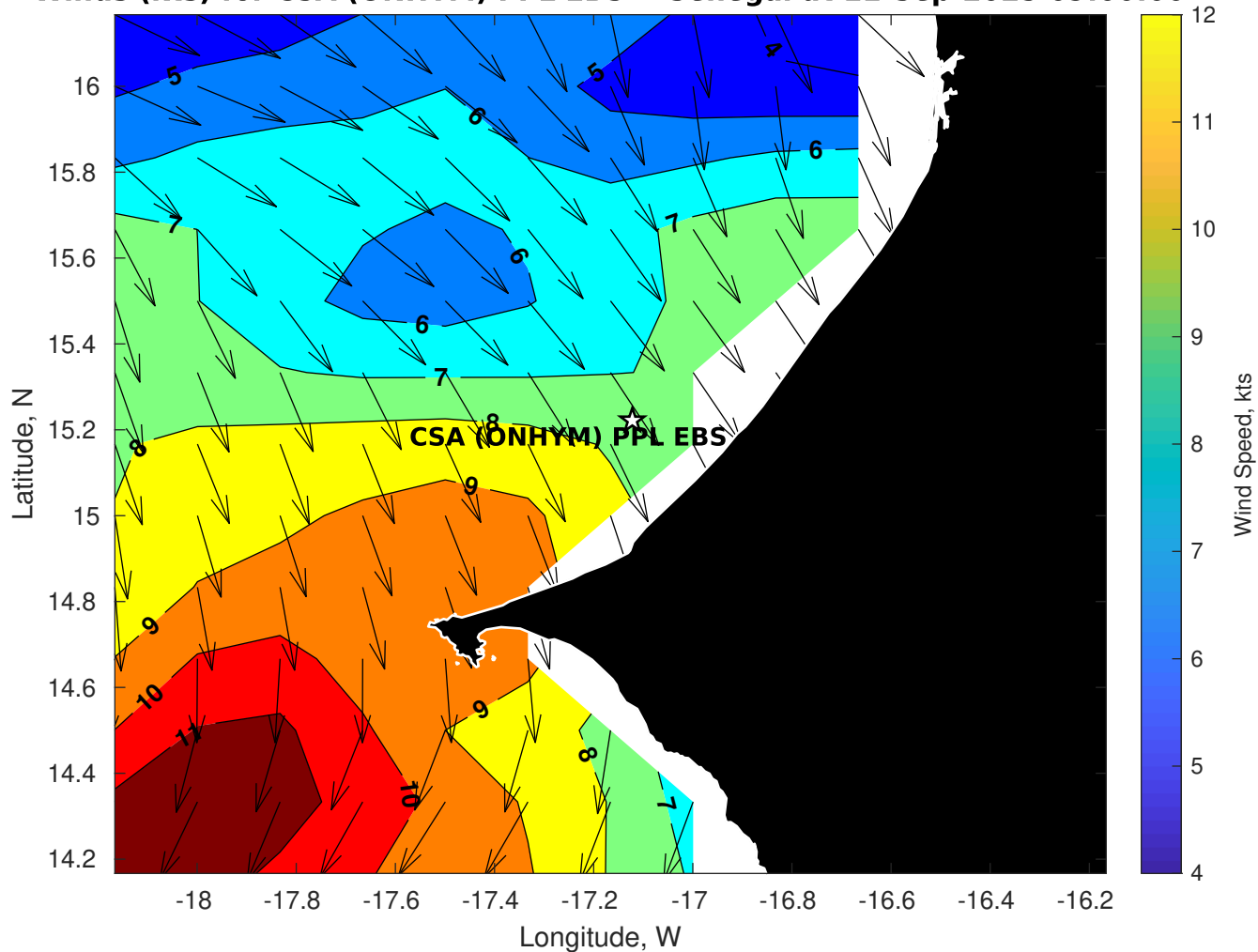
Winds (kts) for CSA (ONHYM) PPL EBS - Senegal at 11-Sep-2025 09:00:00
