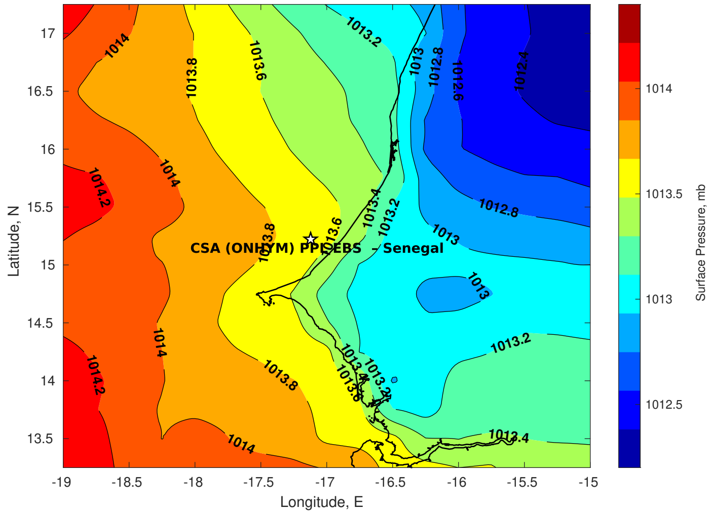
Surface Pressure (mb) for CSA (ONHYM) PPL EBS - Senegal at 12-Sep-2025 12:00:00
