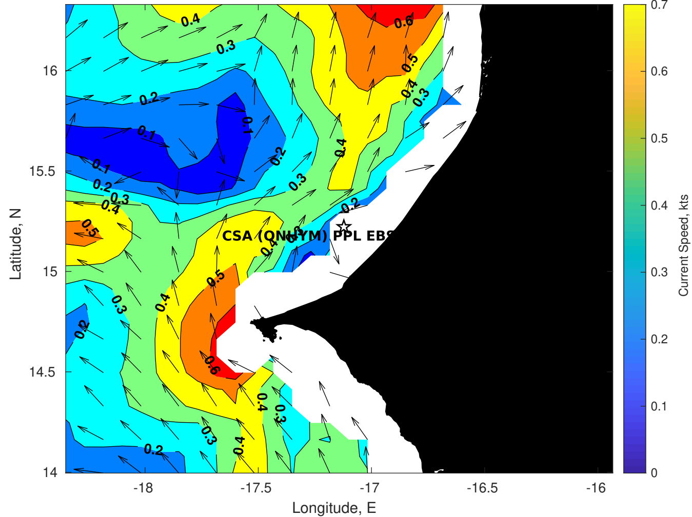
Surface Currents for CSA (ONHYM) PPL EBS - Senegal at 10-Sep-2025 00:00:00
