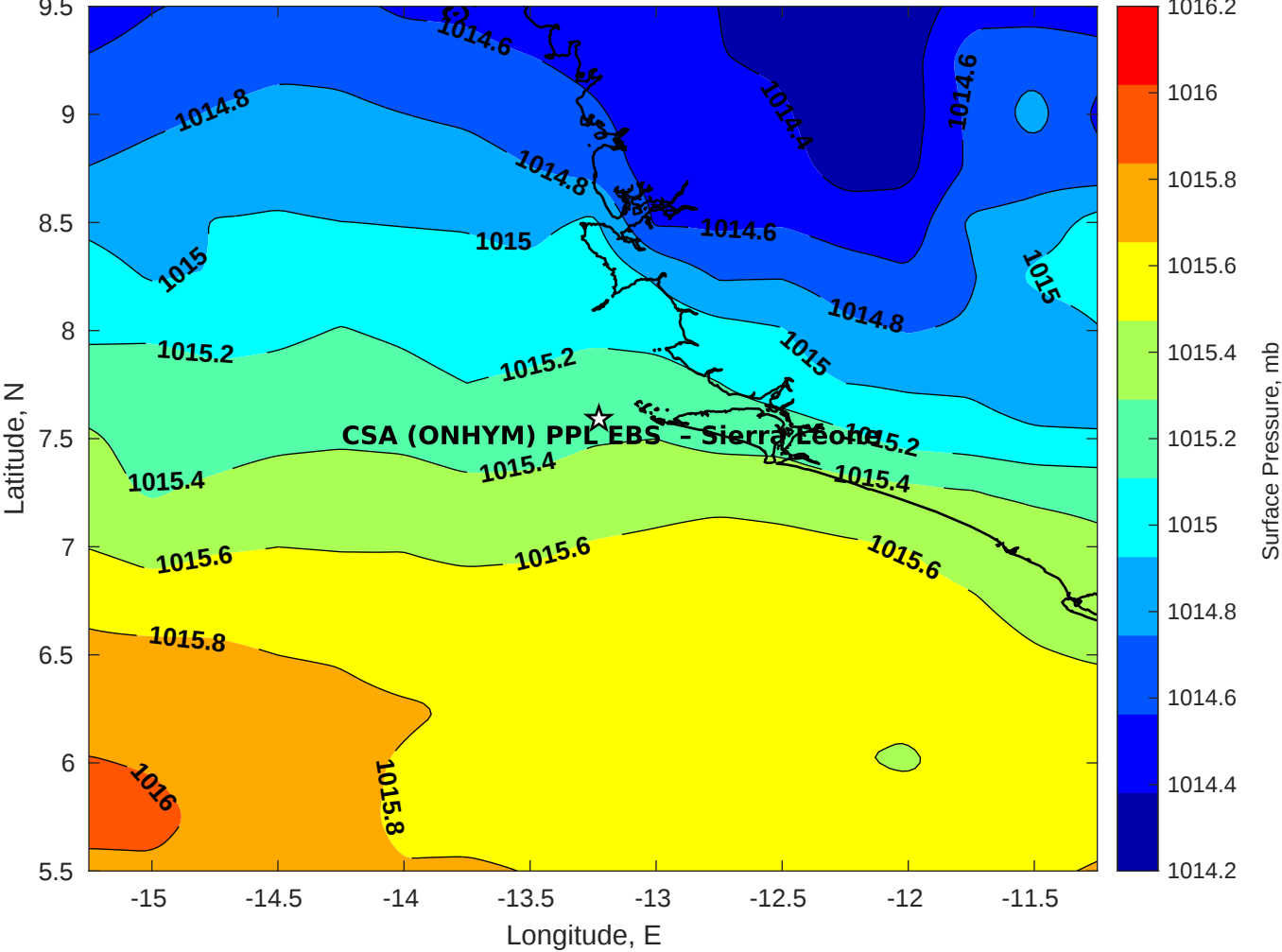
Surface Pressure (mb) for CSA (ONHYM) PPL EBS - Sierra Leone at 12-Sep-2025 12:00:00
